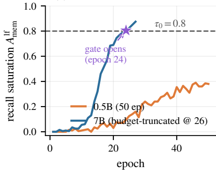
(a) Likelihood recall saturation
