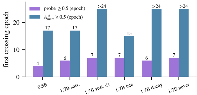
(b) the probe's head start (per run)
