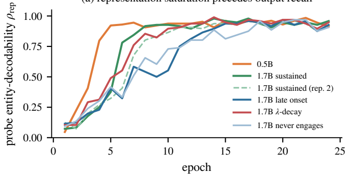
(a) representation saturation precedes output recall
