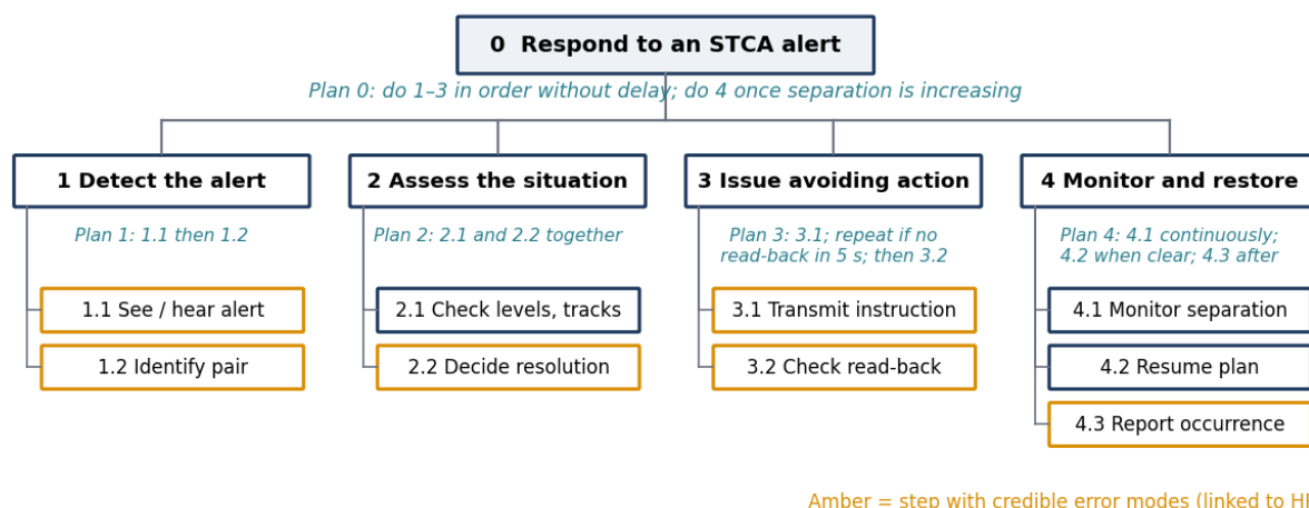
Figure 16. HTA for responding to an STCA alert, with the plans and the steps that carry credible error modes (ARAP HTA module).
