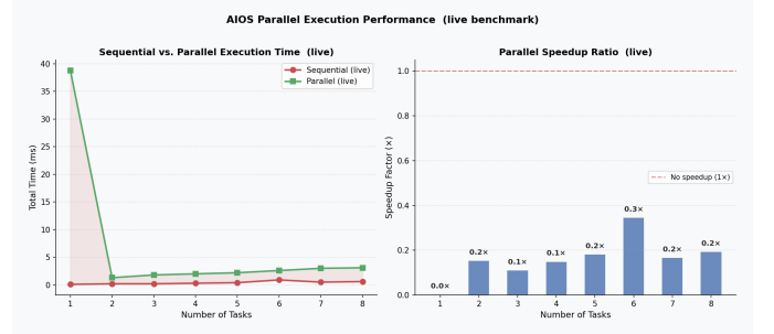
Fig. 3. Parallel Execution Benchmark. Left: total wall-clock time for sequential versus parallel task dispatch as task count scales from 1 to 8. Right: measured speedup ratio (parallel/sequential), showing that thread-pool overhead dominates for microbenchmark tasks but concurrency benefits emerge in real application-launch workloads.
