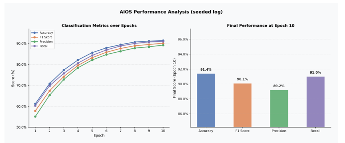
Fig. 4. AIOS intent classification performance. Left: accuracy, F1, precision, and recall over 10 training epochs. Right: final metric values at epoch 10 showing accuracy of 91.4% and F1 of 90.1%.
