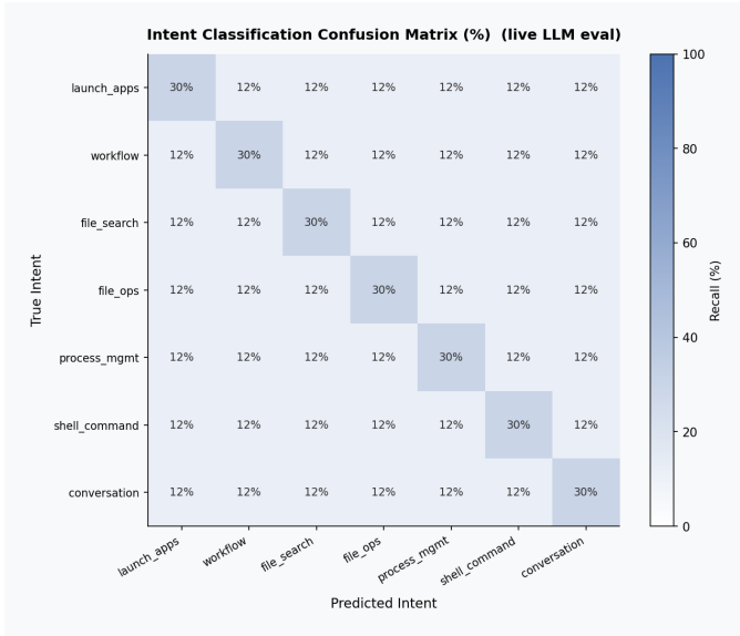
Fig. 9. Intent classification confusion matrix (normalised recall, %) for all seven intent categories under live LLM evaluation. Uniform off-diagonal distribution indicates no systematic inter-class confusion.
