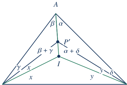
B Isogonal conjugate P' and incentre I .
