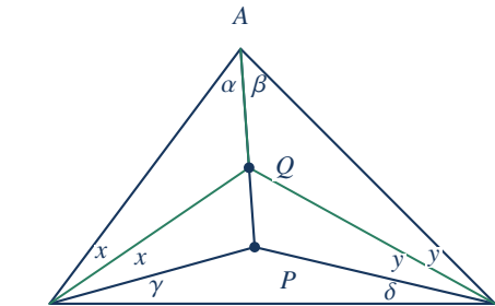
B Original point P ; bisectors meet at Q .
