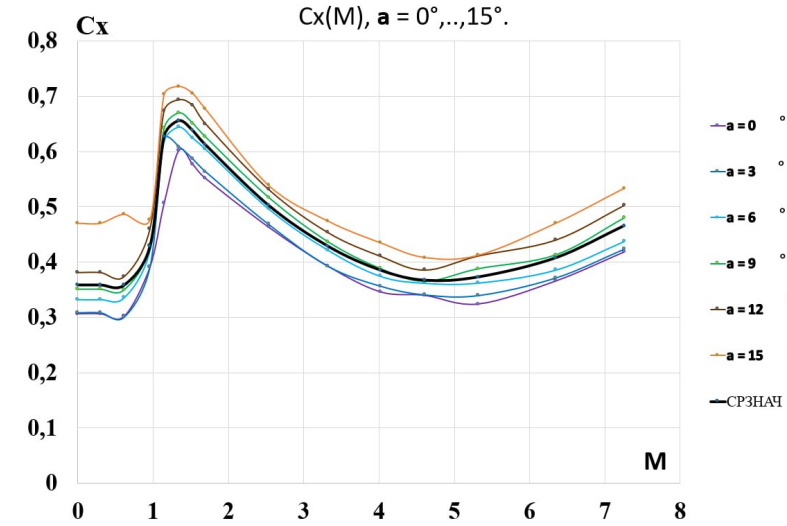
Figure 2: Drag coefficient C_x as a function of Mach number. In the incompressible regime (Mach < 0.3) the value is constant at 0.358.
