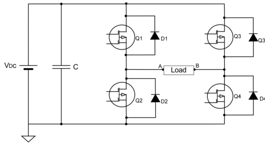
Fig. 7. Full-Bridge topology circuit with four MOSFET operation, where points A and B indicate the load connection.
