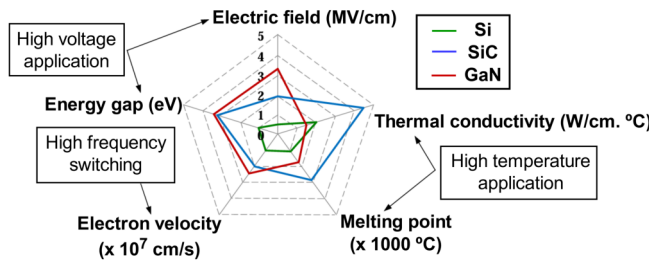
Fig. 1. Comparison of the material properties of Si and SiC. Adapted from [3].
