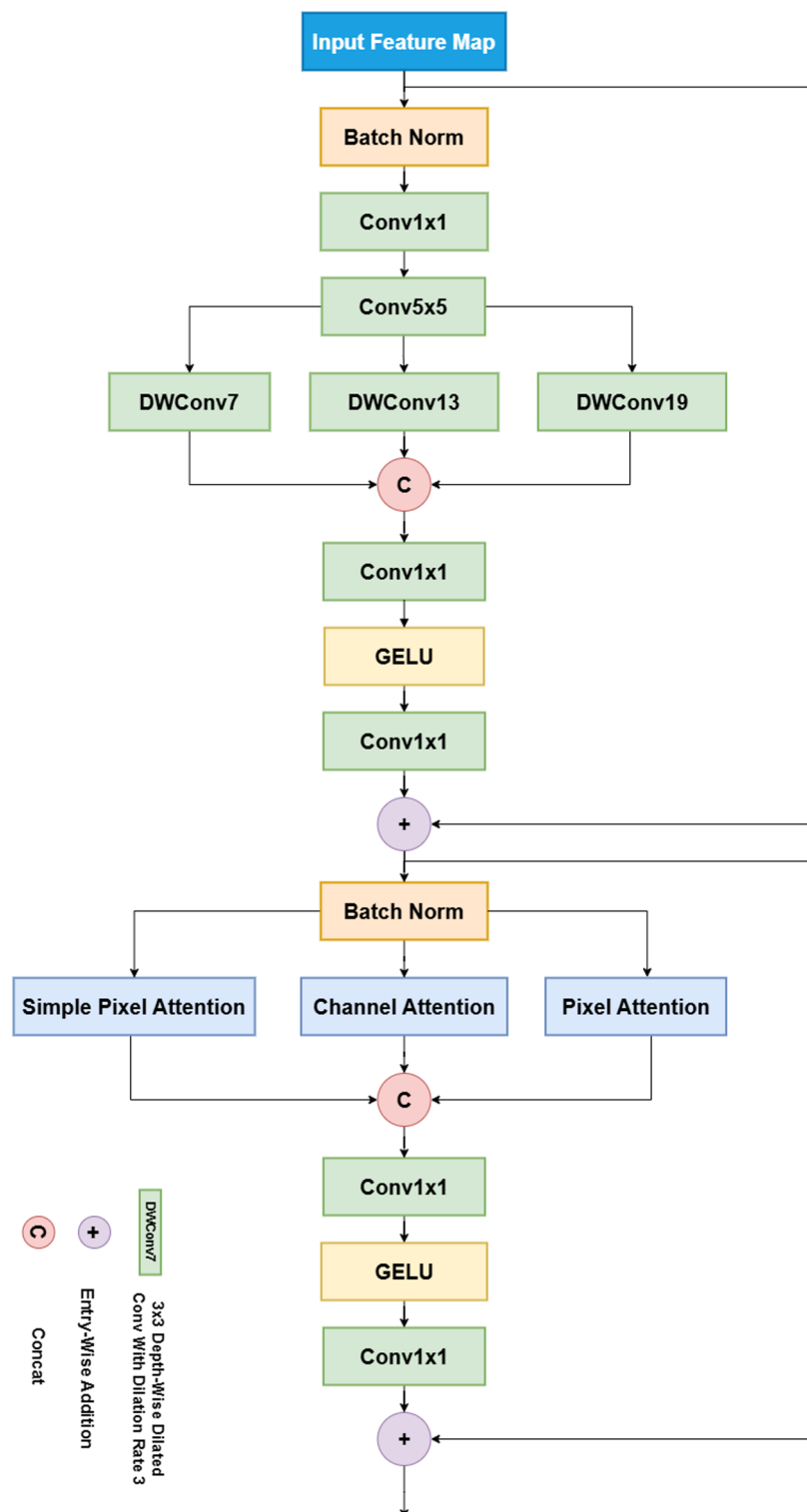
Fig. 2. The framework of MixStructureBlock.
