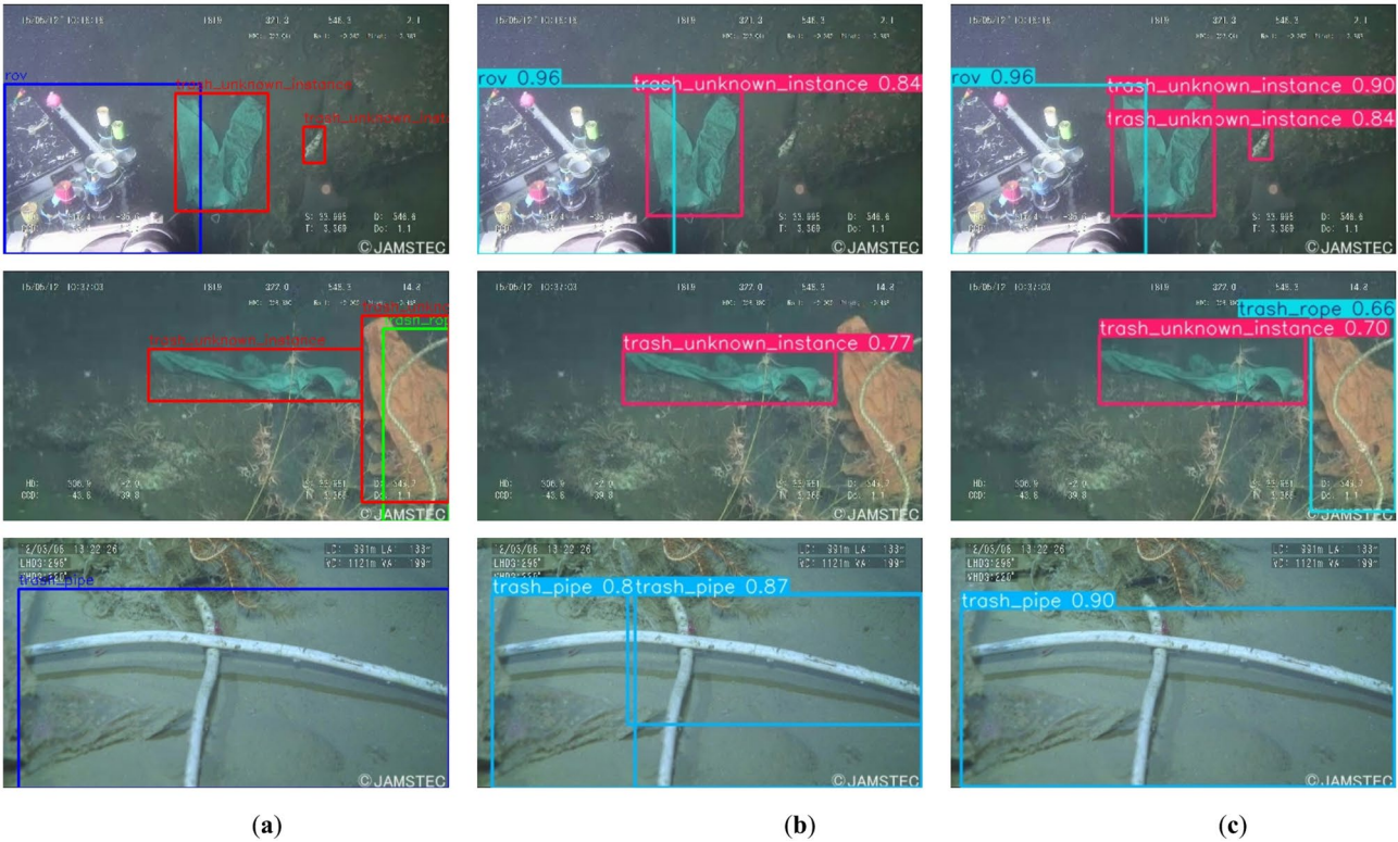
Fig. 5. Detection of YOLOv11 and our model on TrashCan-Instance: (a) True label; (b) YOLOv11; (c) Our model.
