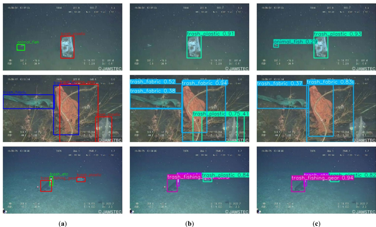
Fig. 6. Detection of YOLOv11 and our model on TrashCan-Material: (a) True label; (b) YOLOv11; (c) Our model.
