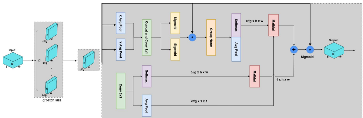
Fig. 3. The framework of EMA.
