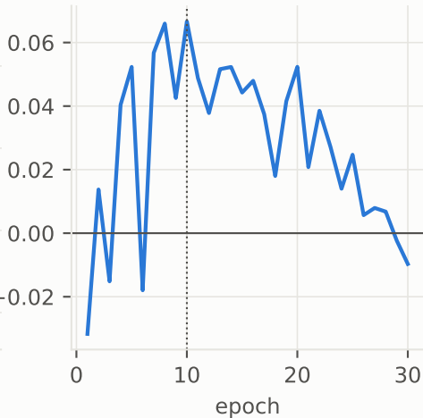
Validation rank-IC
