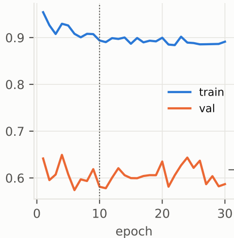
MTL loss
