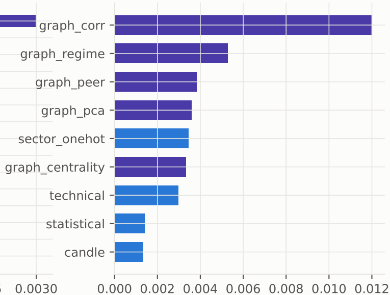
Importance by feature group
