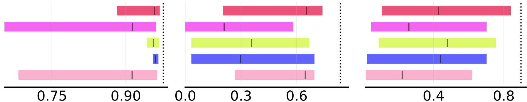
IQM finger-spin
