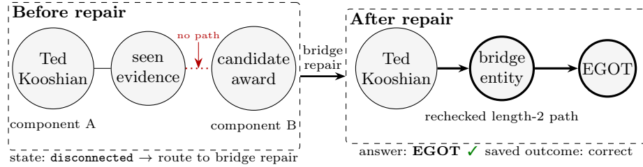
Fig. 2. Replayable Repair Trace for a representative saved case. The question, graph state, repair, reader route, and answer are all recoverable from saved fields, so the before/after repair decision can be audited without regeneration.
