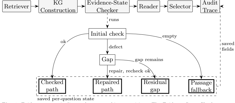
Fig. 1. Evidence-state pipeline and state-machine transitions. The Evidence-State Checker runs a structural state machine whose terminal state is saved per-question and written to the audit trace for replayable inspection.
