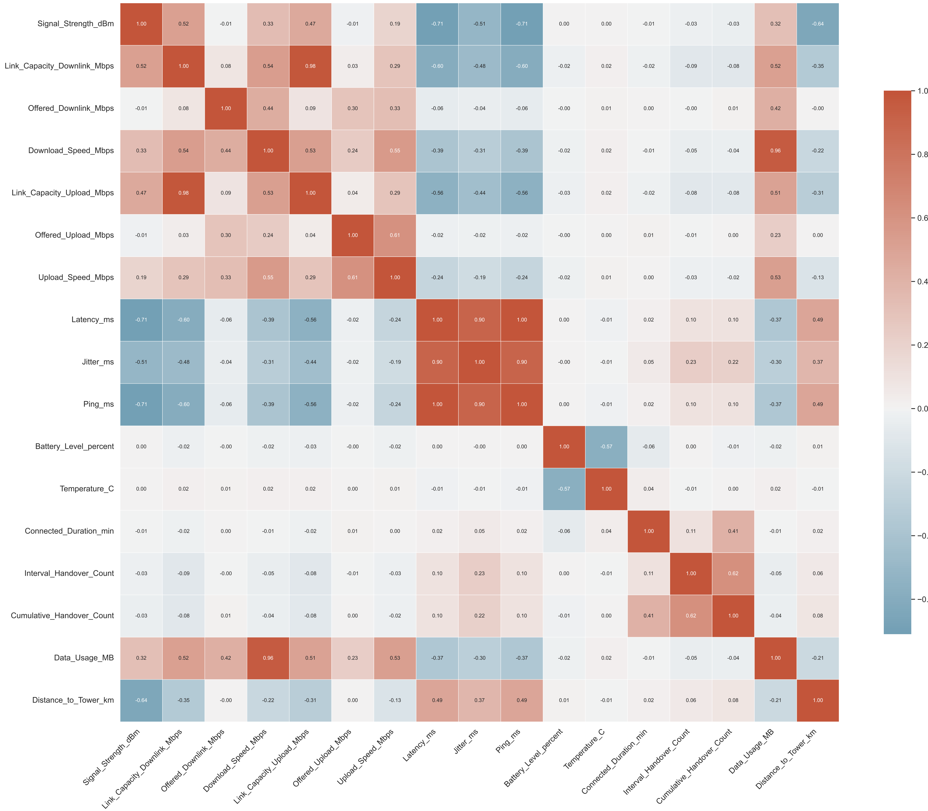
Primary Synthetic QoS Parameters Correlation
