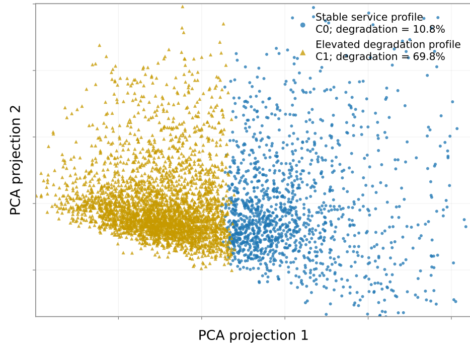
(a) Reduced-context K-Means profiles
