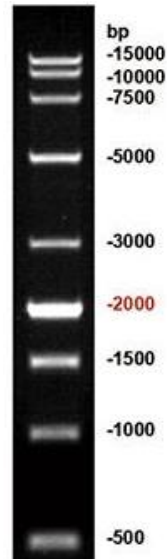
GN15K DNA Marker
