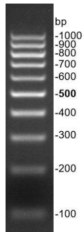
GN100bp DNA Ladder III
