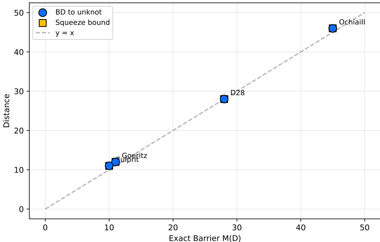
Bottleneck Distance to Unknot vs M(D) r = 1.000
