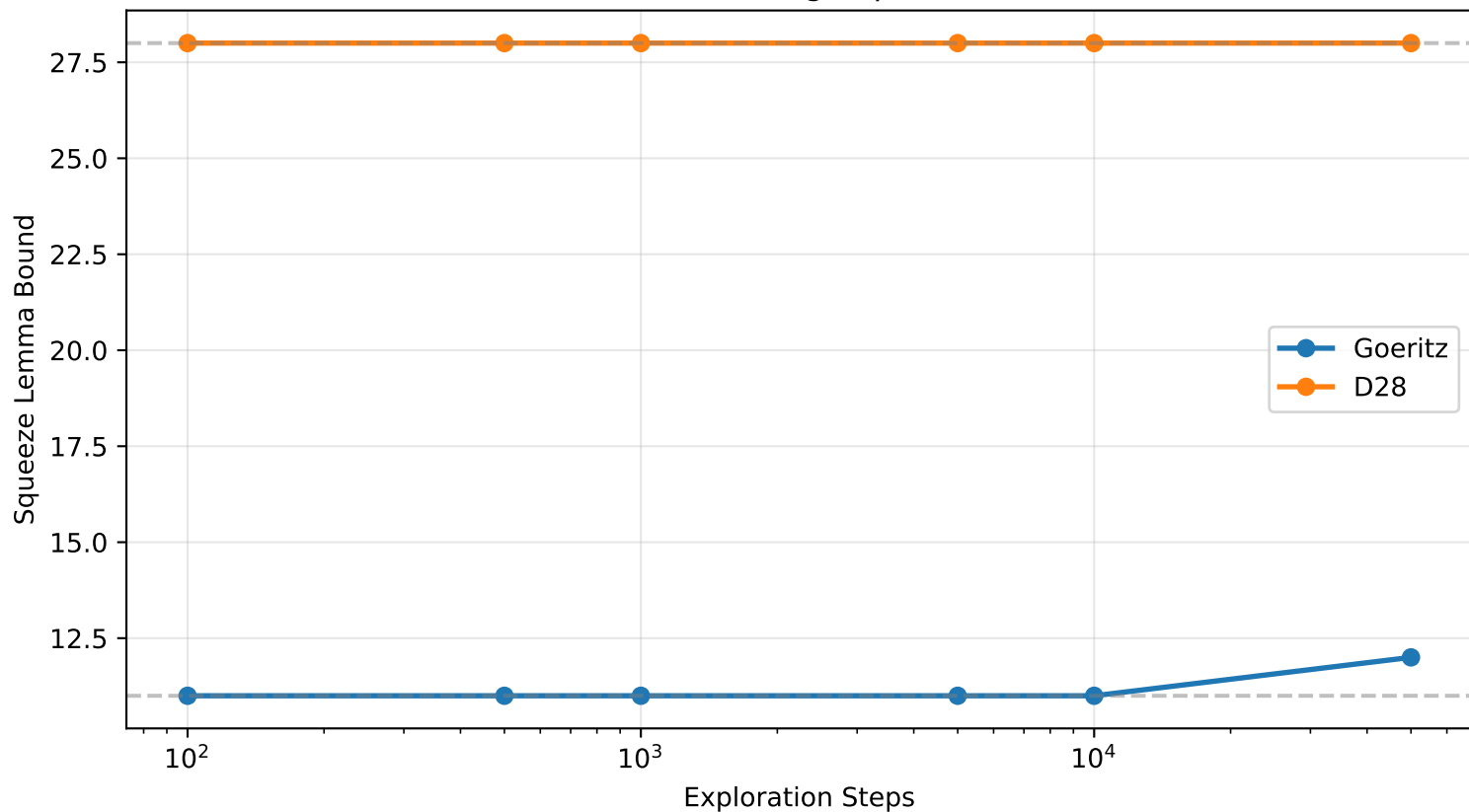
Convergence of Squeeze Lemma Bound with Increasing Exploration
