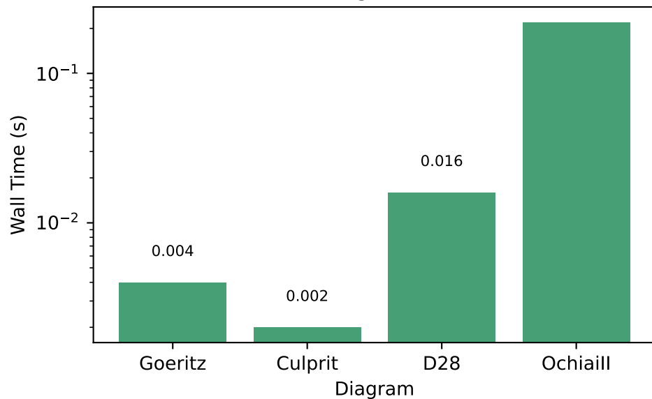
BFS Runtime (at ceiling N = \text{cr}(D) )
