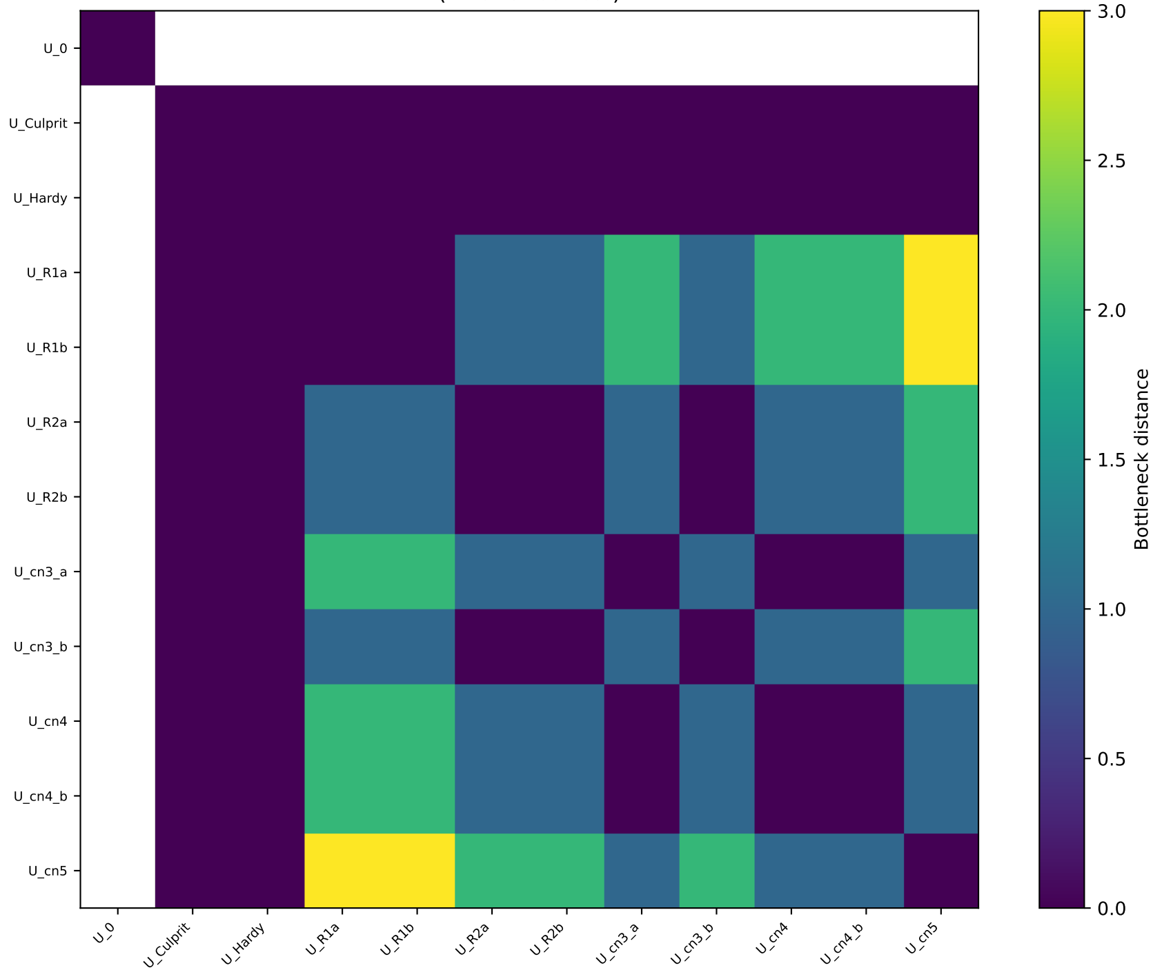
Bottleneck Distances Between Unknot Diagrams (Invariance Test)
