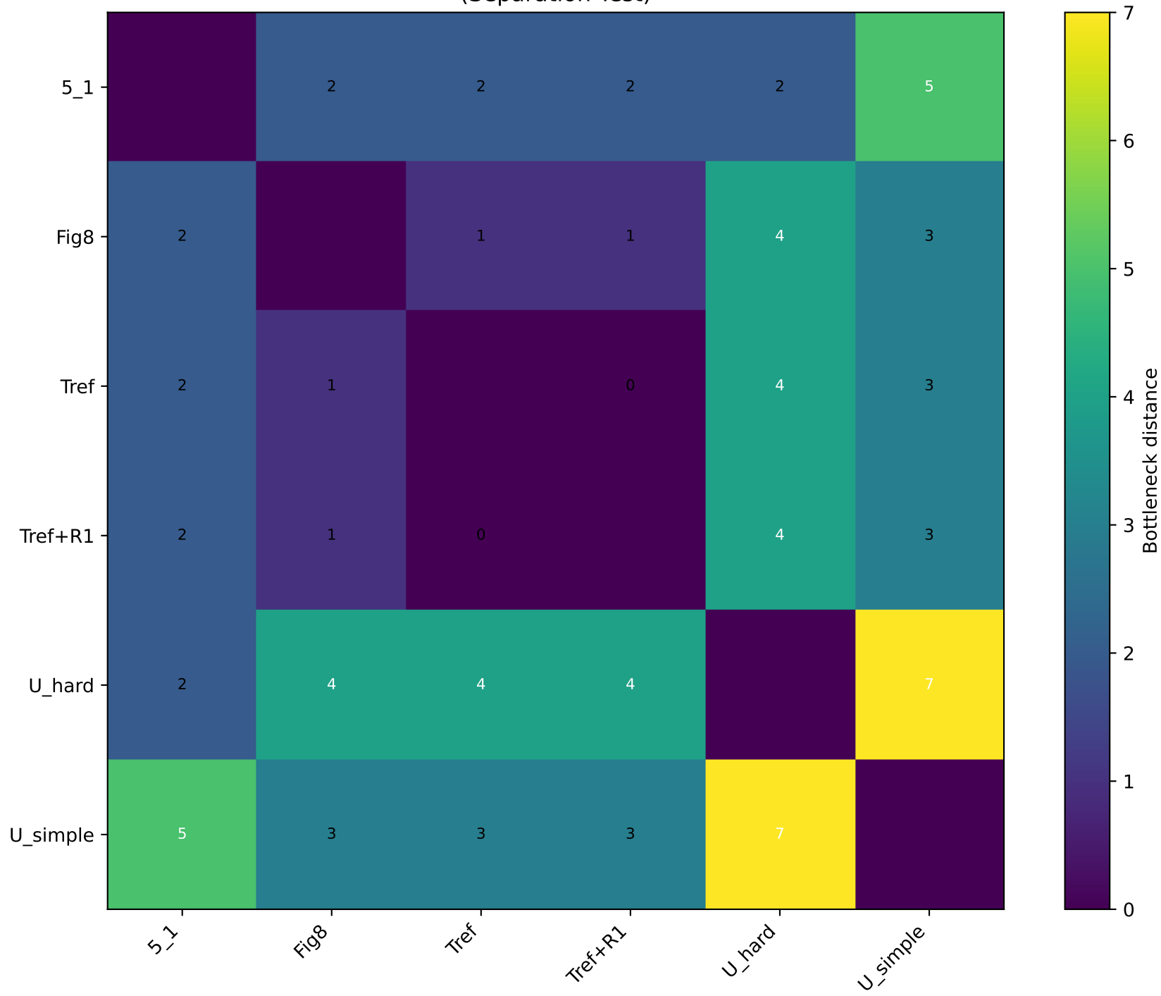
Bottleneck Distances Between Knot Diagrams (Separation Test)
