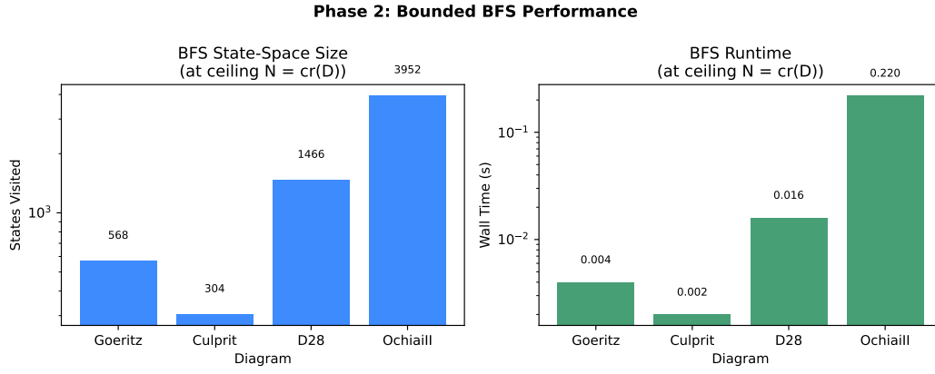
■ Figure 1 BFS state-space size and runtime for the four hard unknot diagrams at ceiling N = \text{cr}(D) . Both axes are logarithmic. The algorithm visits fewer than 4 000 states and completes in under one second for all four diagrams.
