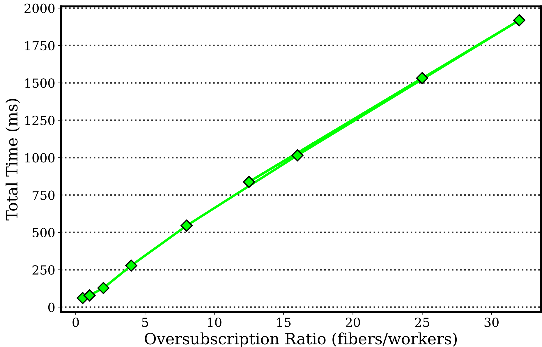
Total Execution Time vs Oversubscription
