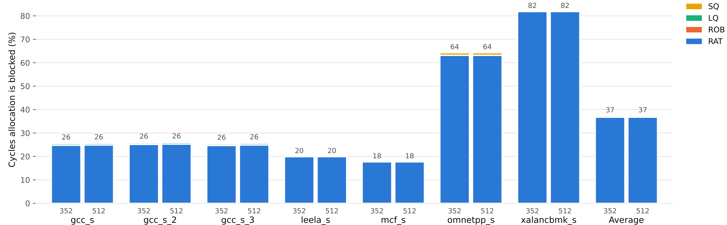
Backend stalls by resource
