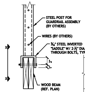
SECTION ⑦
