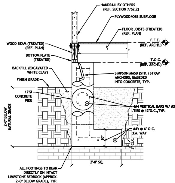
PIER & BEAM, TYP. TYPE F2/F3 ①
