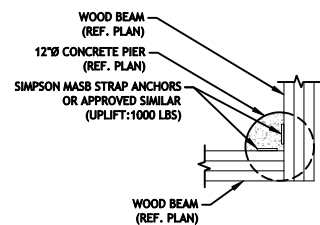
DETAIL ⑤
