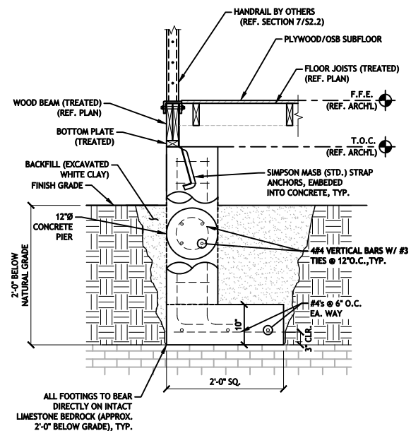
PIER & BEAM, TYP. TYPE F2/F3 ②
