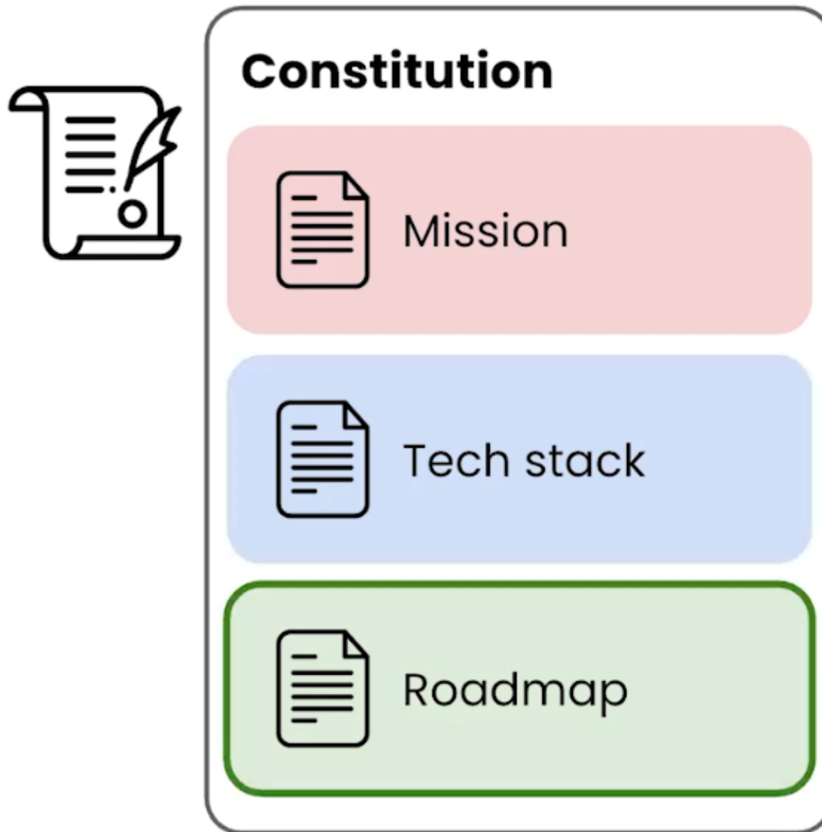
Figure 39.1: Constitution
