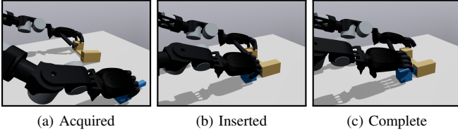
Fig. 4. Assembly Sequence. Both one-step selectors produce these states at friction \theta = 0.7 . Physical finger contacts support acquisition and transport. Completion follows table support, hand withdrawal, and two seconds of stationary dwell.
