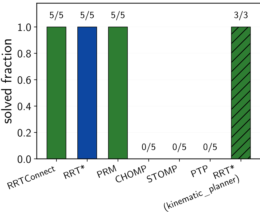
Success rate
