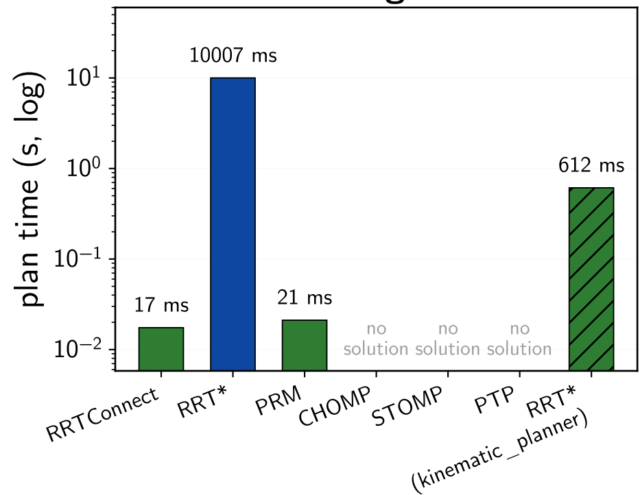
Planning time
