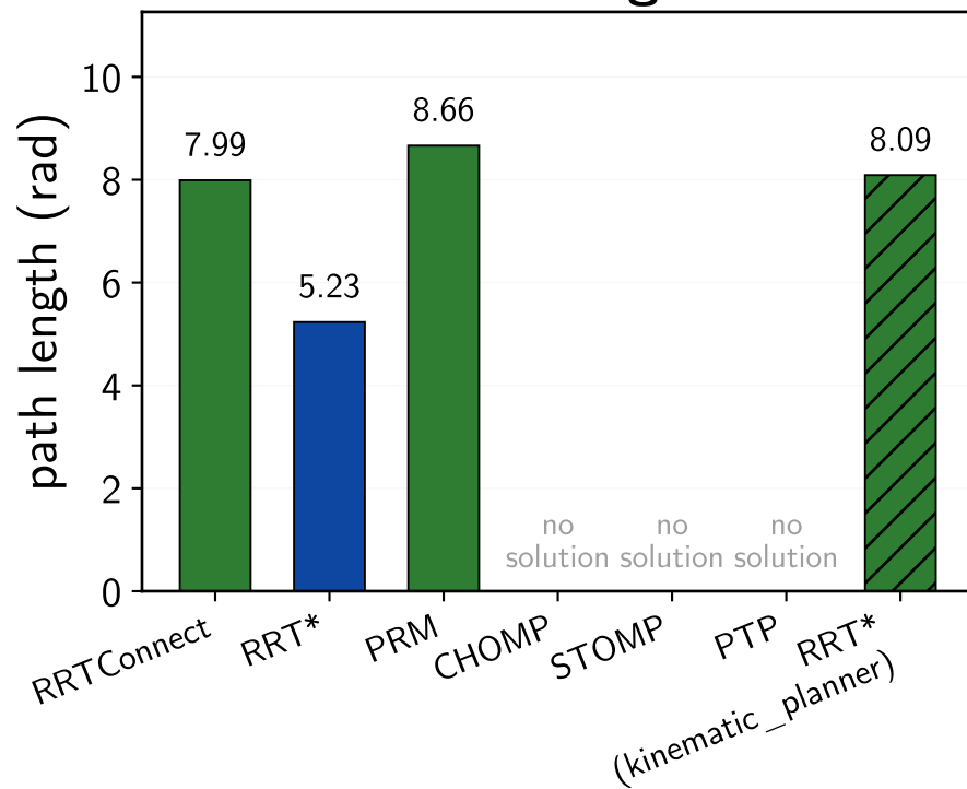
Path length
