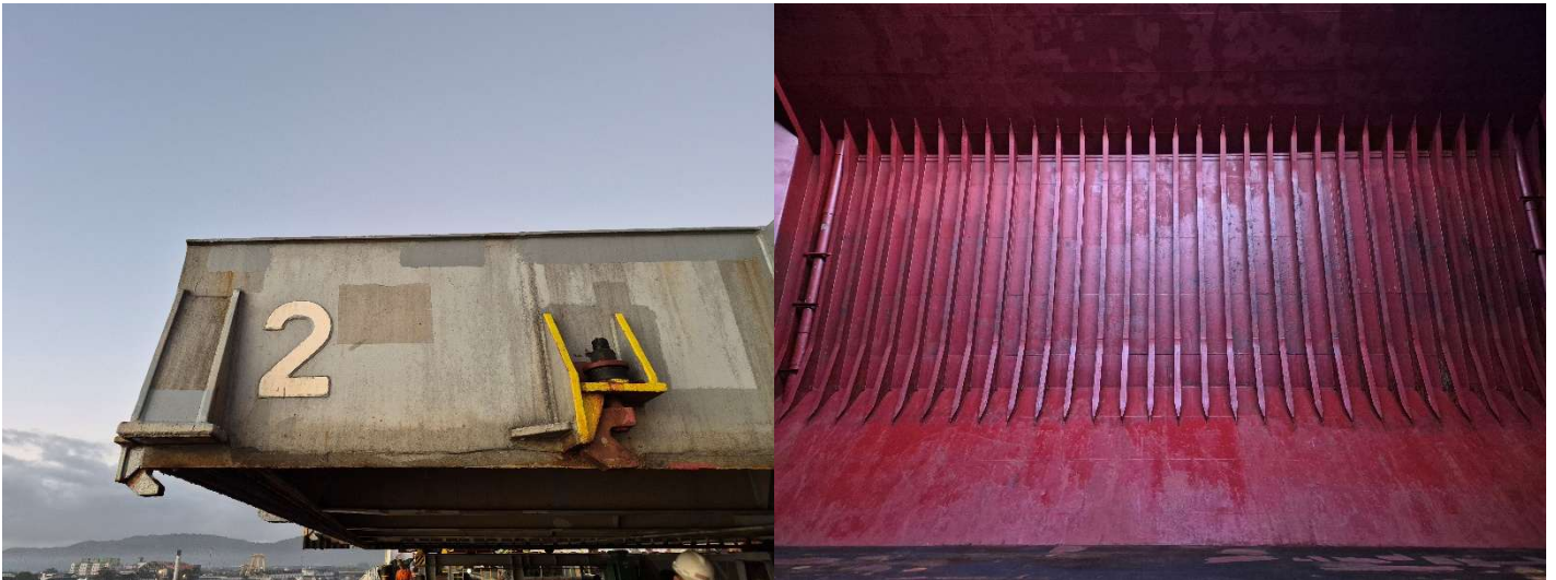
Holds inspection #2
