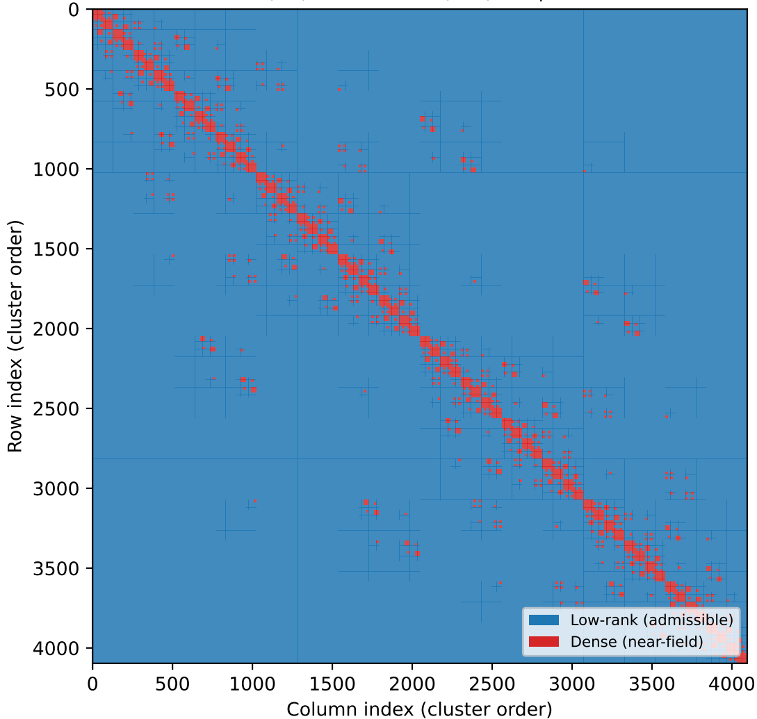
H-matrix block structure N_s = 64 , N = 4096 2116 dense (red), 6900 low-rank (blue), compression 0.314x
