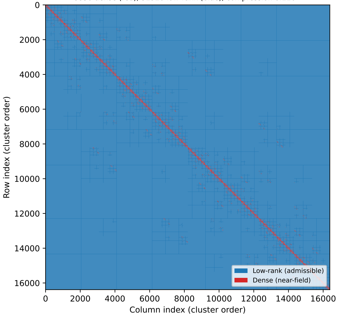
H-matrix block structure N_s = 128 , N = 16384 8836 dense (red), 31920 low-rank (blue), compression 0.116×
