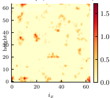
Pressure p (H-matrix BEM)
