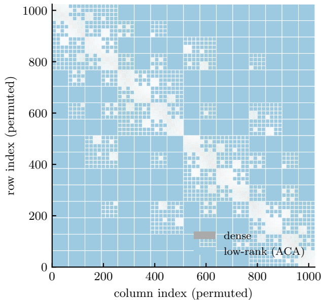
H-matrix block structure, N_s = 32
