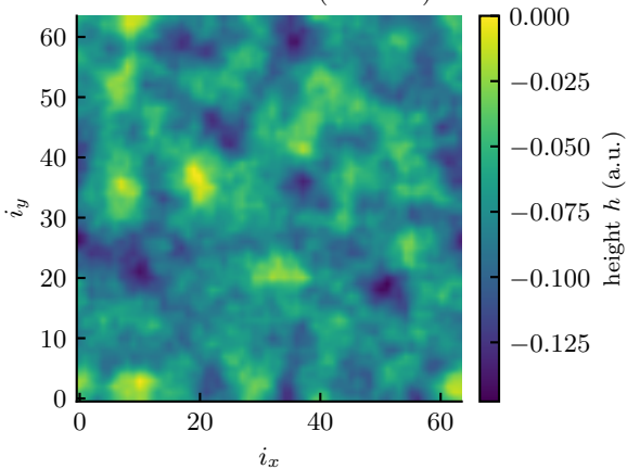
Self-affine surface ( H = 0.8 )
