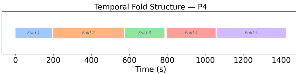
Figure 3.19: Temporal minimum required safety distance of 3 seconds between train and test windows is strictly fulfilled.
