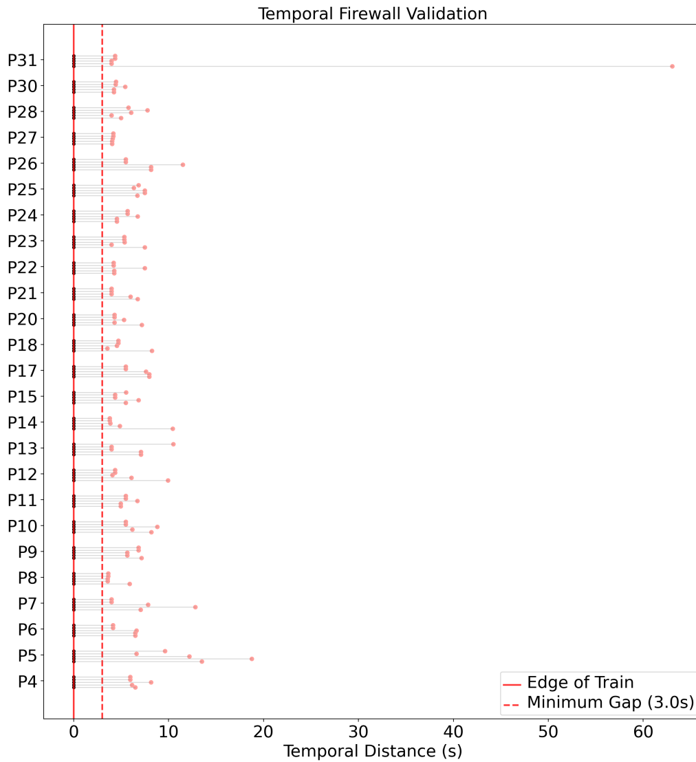
Figure 3.19: Temporal minimum required safety distance of 3 seconds between train and test windows is strictly fulfilled.
