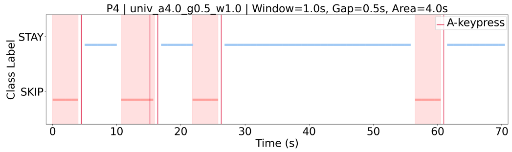
Figure 3.8: Window parameter exploration (default parameters, except a smaller gap size & a longer imminent-skip period (Skip-Area)).
