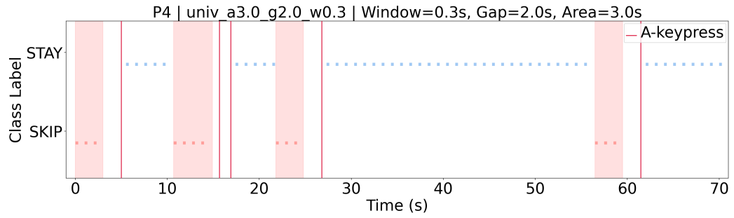
Figure 3.7: Window parameter exploration (default parameters, except a smaller window size).
