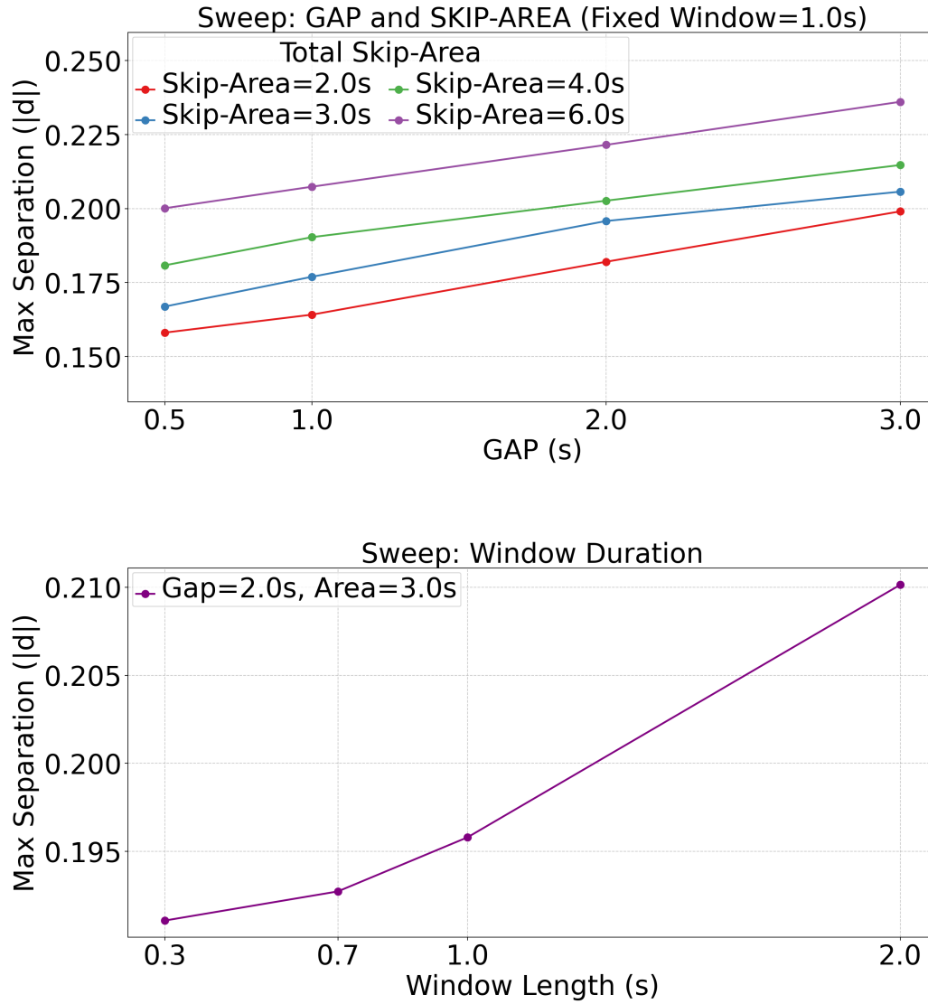
Figure 3.9: Parameter sweep of the window exploration analysis. The sweep evaluates only individual component features and does not use the Engagement Index.
