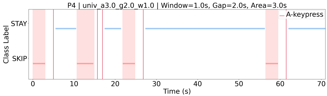
Figure 3.6: Schematic overview of the labeling strategy under the default parameterization. The figure illustrates the placement of the STAY and SKIP labels relative to the registered press markers, including the default gap length, window length, and imminent-skip period.
