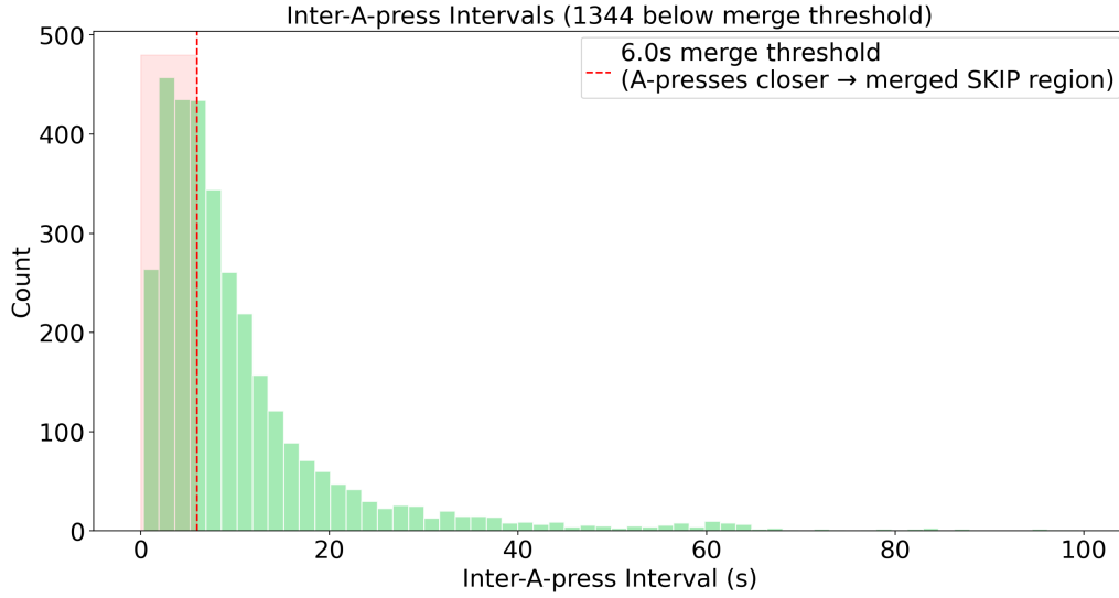
Figure 3.13: Distribution of inter-swipe intervals (view times of each video across all participants, or dwell time). The shaded region highlights intervals below the 6.0-second merge threshold, where consecutive SKIP windows overlap to form behavioral burst blocks.
