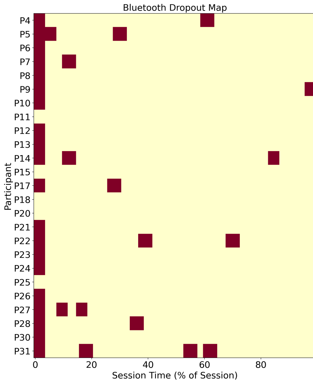
Figure 3.11: Bluetooth Dropout Heatmap indicating signal loss events across the experimental timeline. Data windows overlapping with these dropouts were removed from the analysis pipeline.
