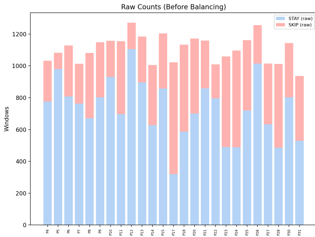
Figure 3.17: Raw window counts before balancing.
