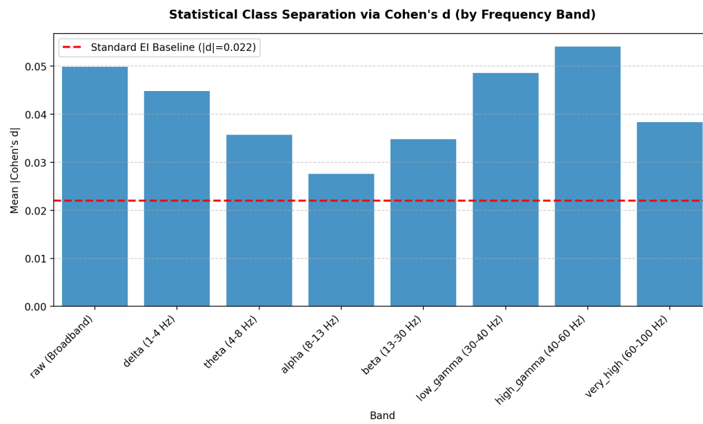
Figure 3.26: Cohen's d effect size by frequency band.
