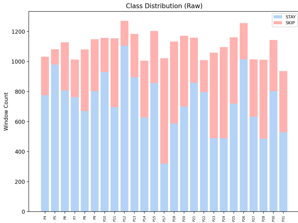
Figure 3.14: Raw class distribution (STAY vs. SKIP) before balancing.
