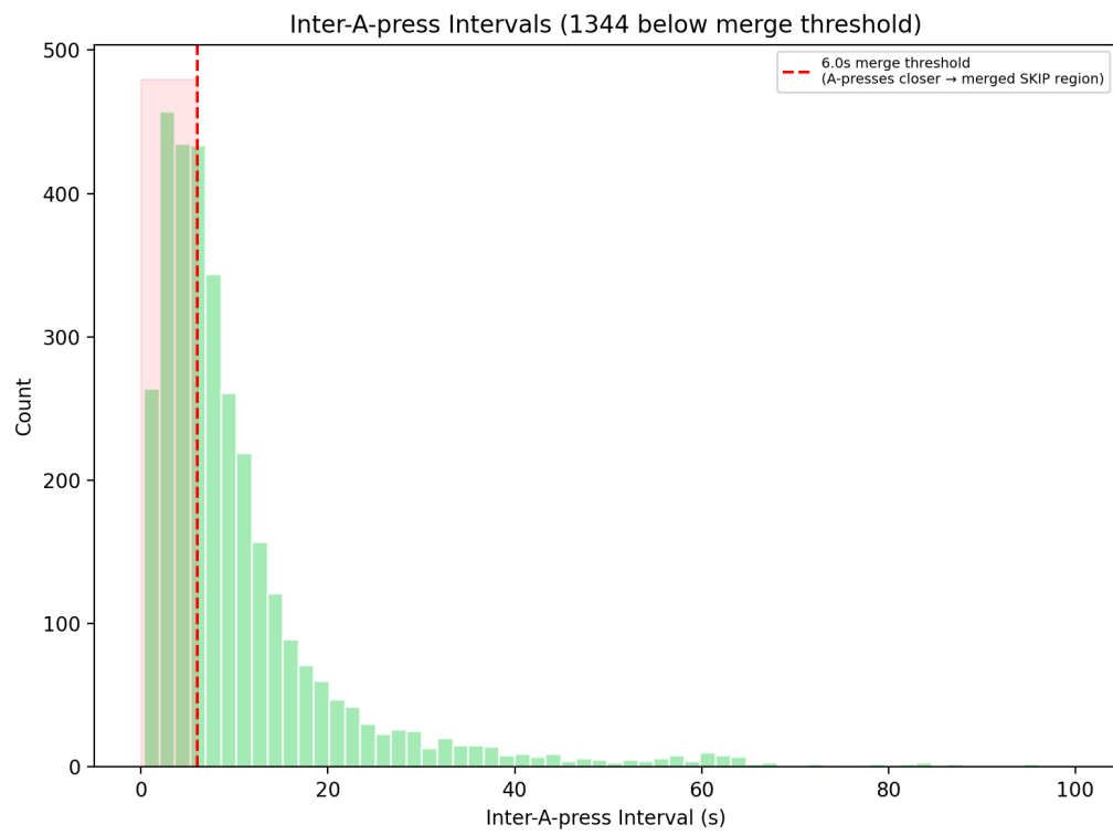
Figure 3.15: Window duration analysis.
