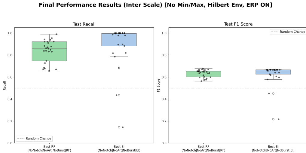
Figure 3.42: Final inter-subject performance summary.
