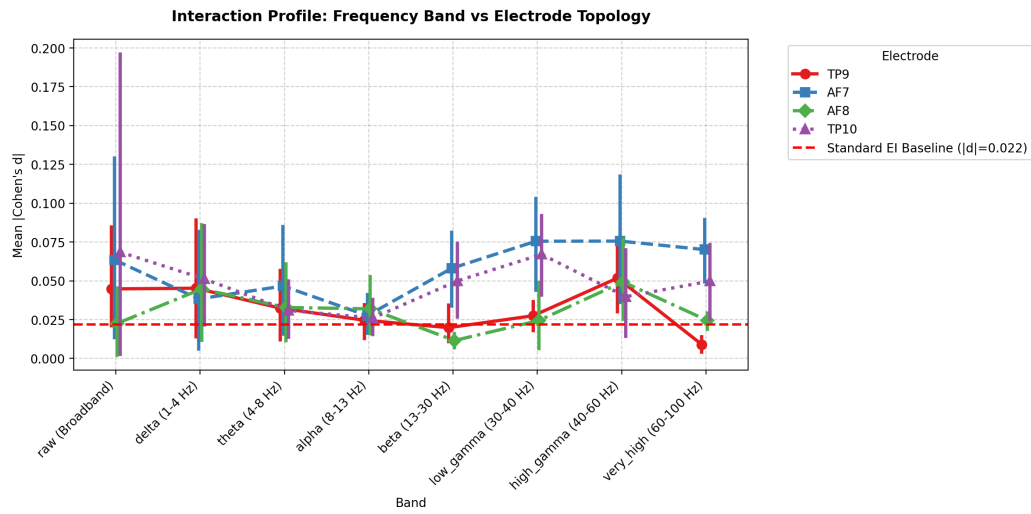
Figure 3.29: Cohen's d effect size interactions.
