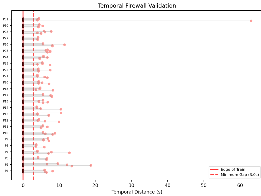
Figure 3.22: Temporal fold separation details.
