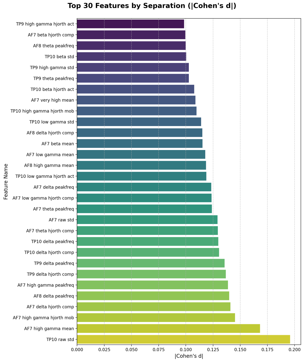
Figure 3.34: Top features ranked by Cohen's d.
