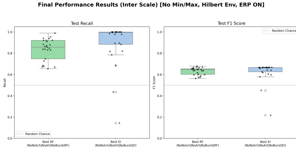
Figure 3.38: Final inter-subject performance summary.
