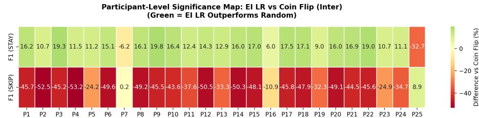
Figure 4.10: Inter-subject significance analysis.
