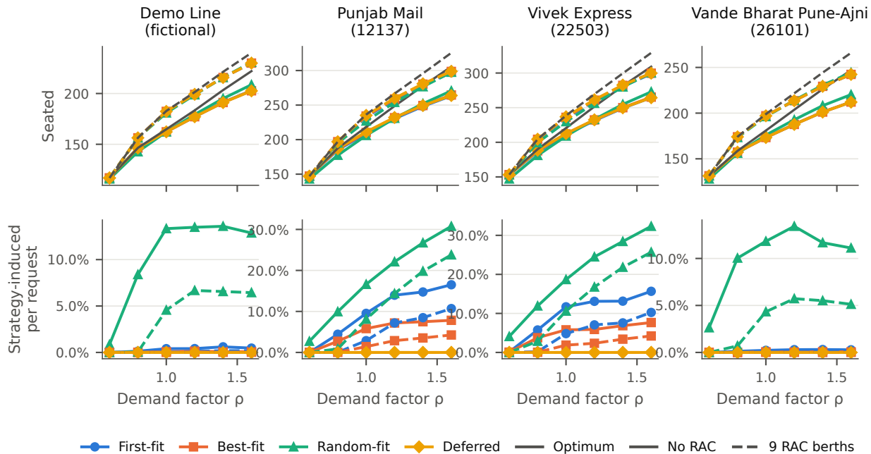
F6. Effect of RAC (mixed trips): solid = no RAC, dashed = 9 RAC berths
