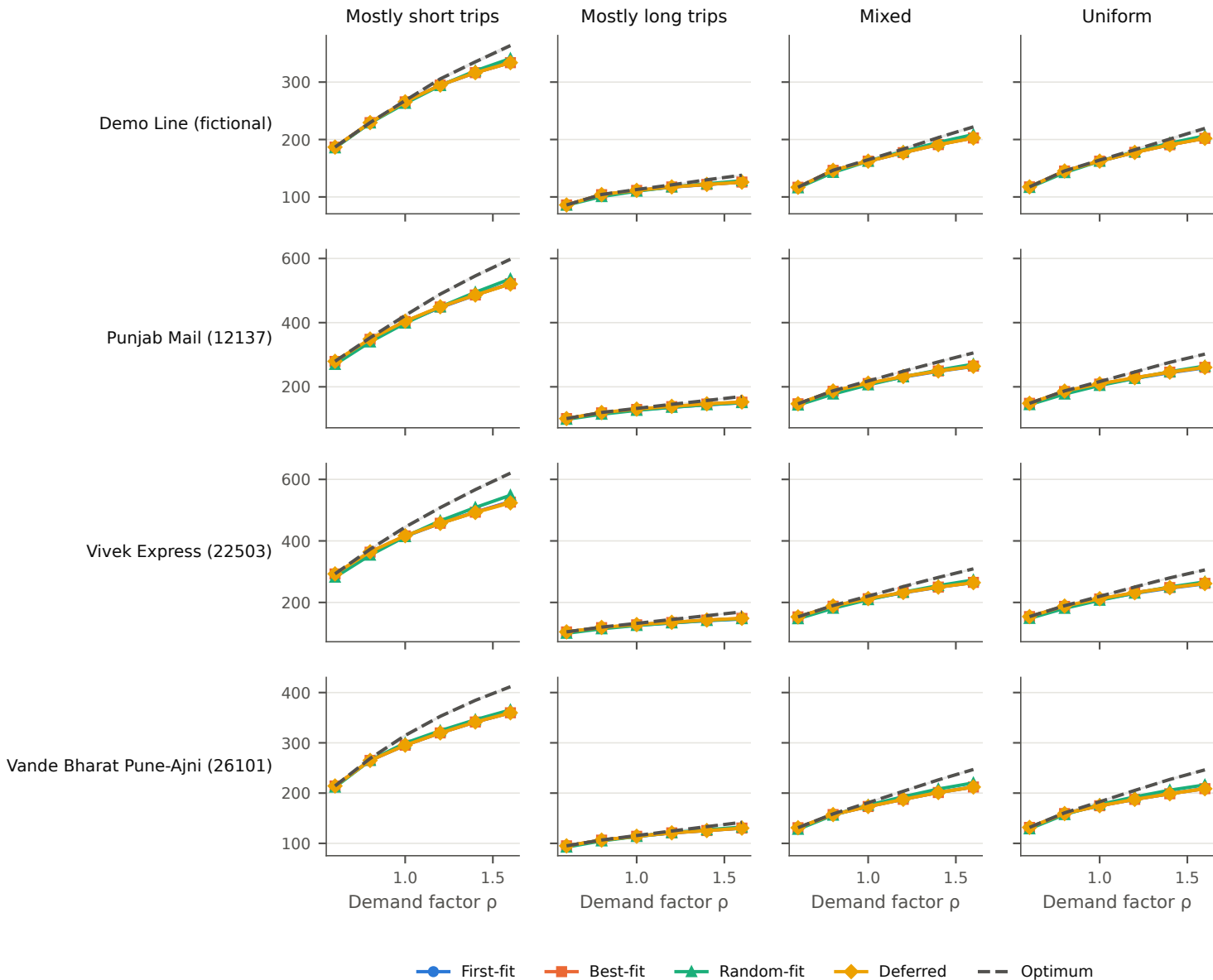
F1. Passengers seated vs demand (mean, 95% CI)
