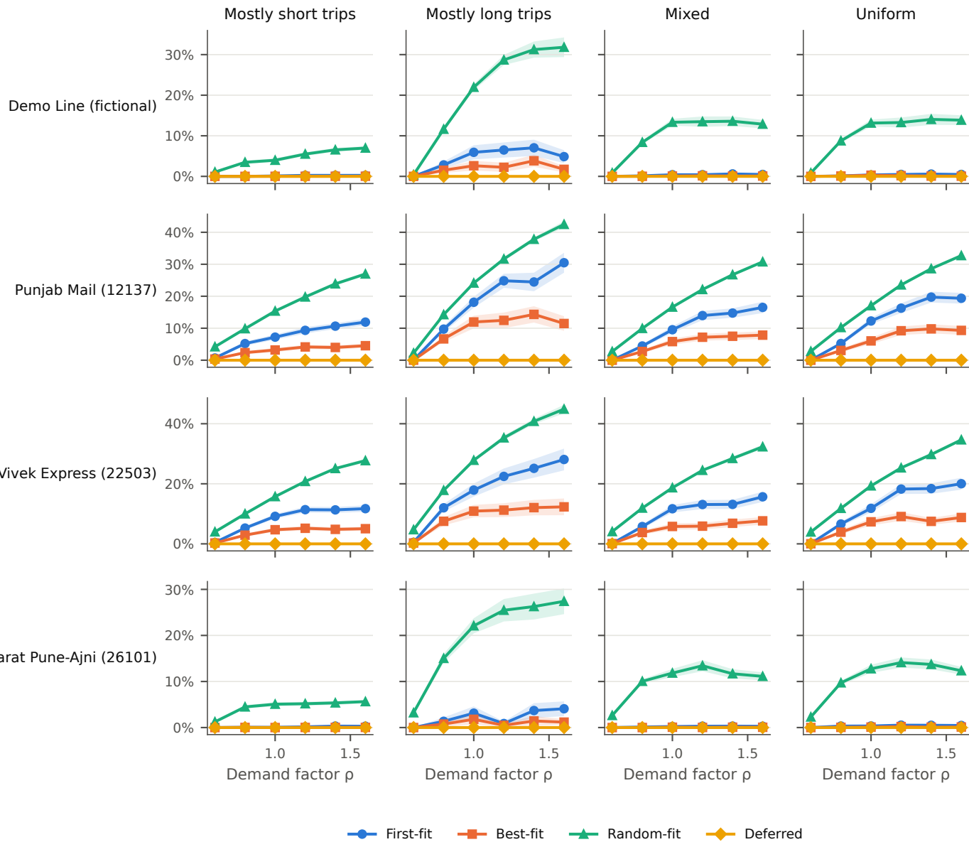
F2. Strategy-induced rejections per request vs demand (mean, 95% CI)
