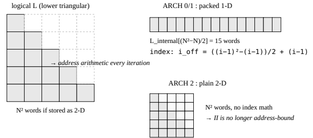
Fig. 3. Memory organisation trade-off in cholesky.hpp . ARCH 2 spends 2x memory to remove the per-iteration address computation that limits the initiation interval.
