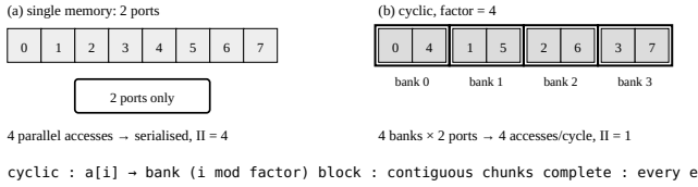
Fig. 14. Array partitioning. Unrolling is legal only when the memory can deliver the required number of accesses per cycle; cyclic partitioning is used when the access stride is one.
