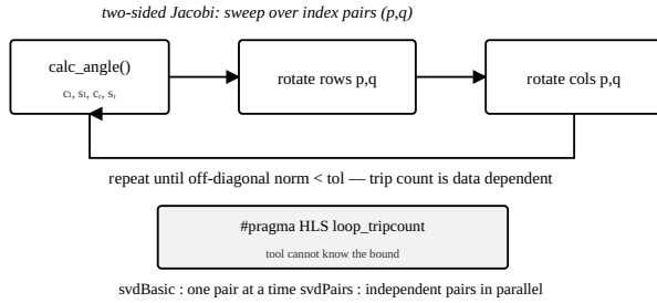
Fig. 6. Two-sided Jacobi SVD in svd.hpp . The iteration count depends on the data, which is why loop_tripcount appears; svdPairs exploits that disjoint index pairs commute.
