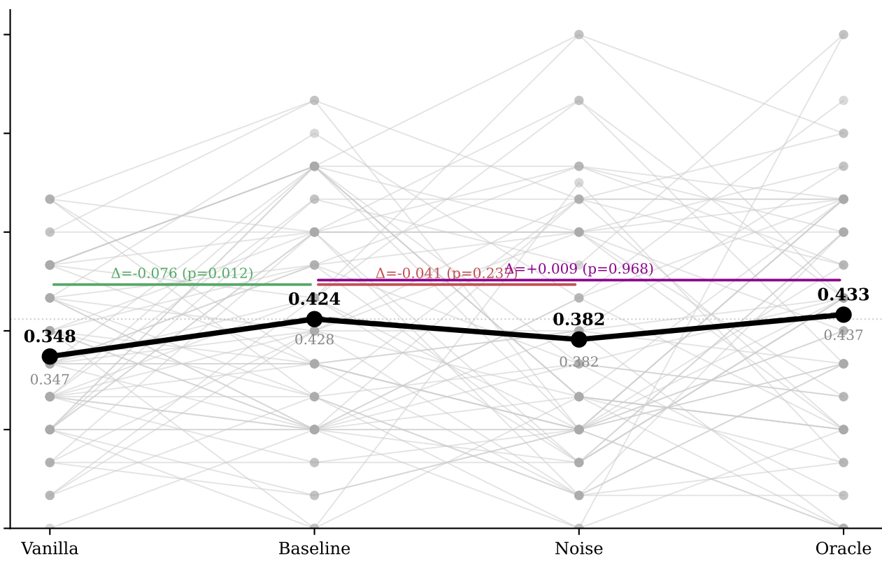
Qwen2.5
