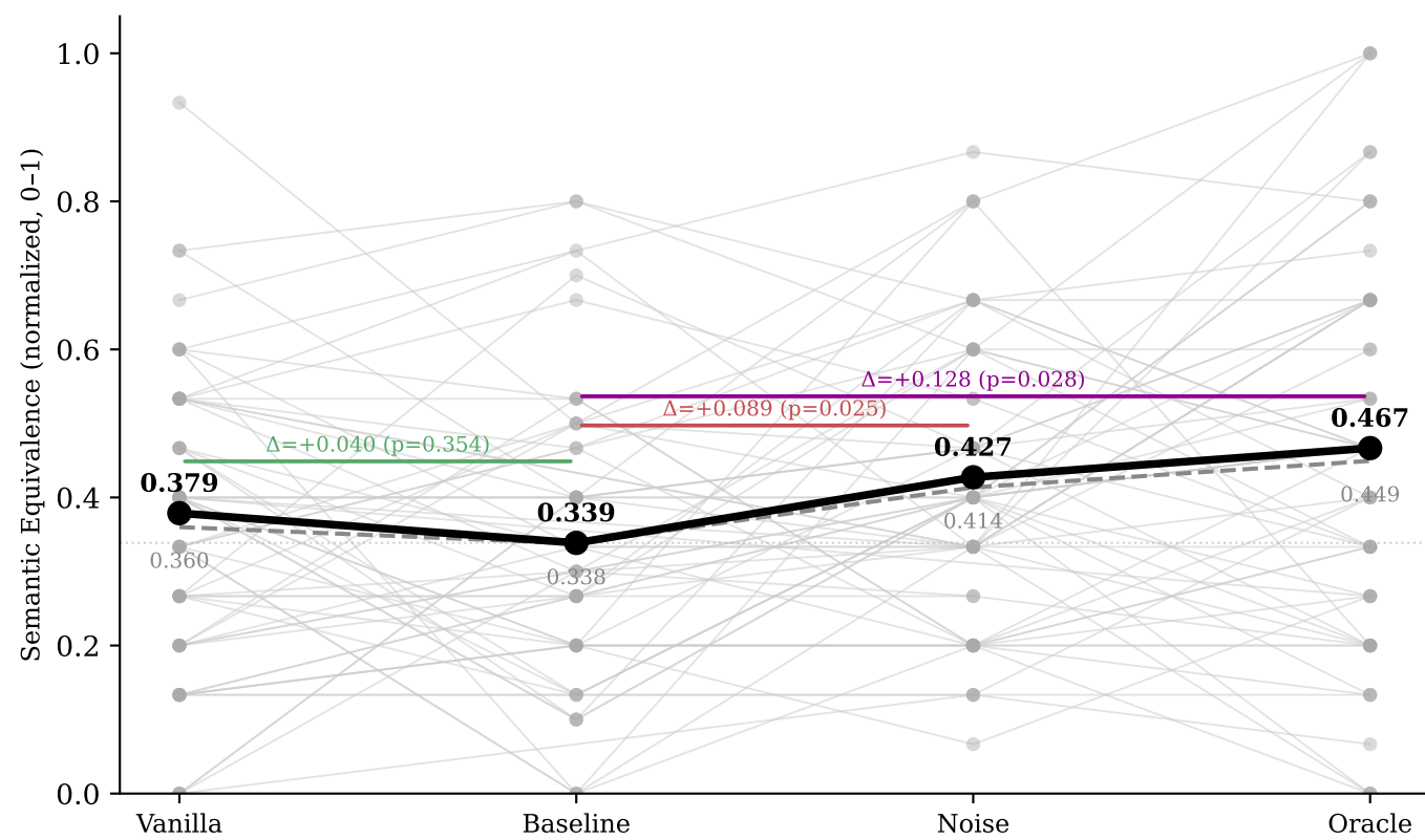
Mistral
