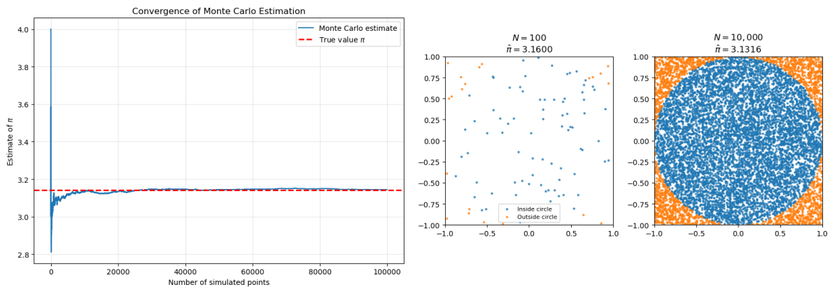
Monte Carlo Estimation of \pi
