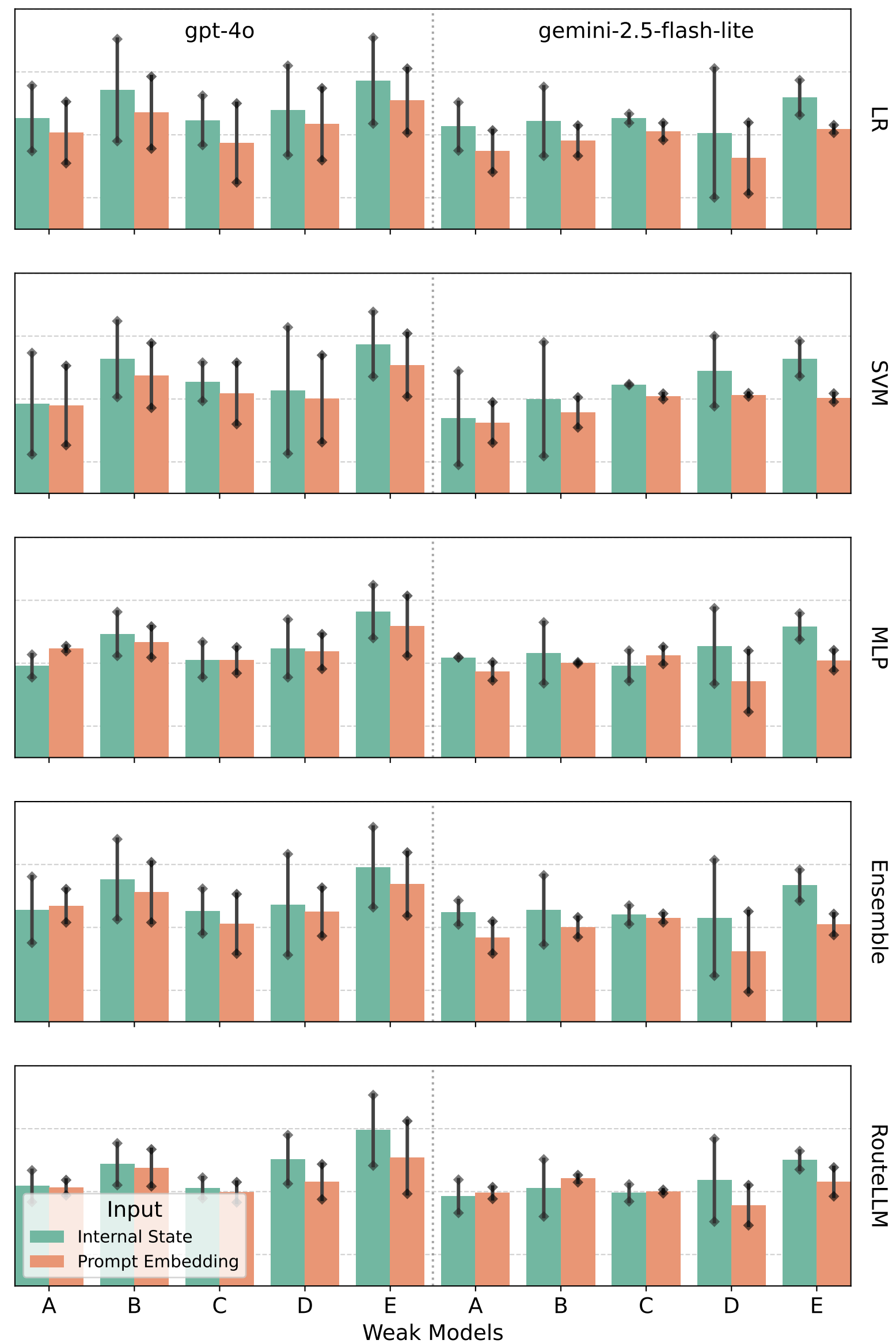
Code Generation
