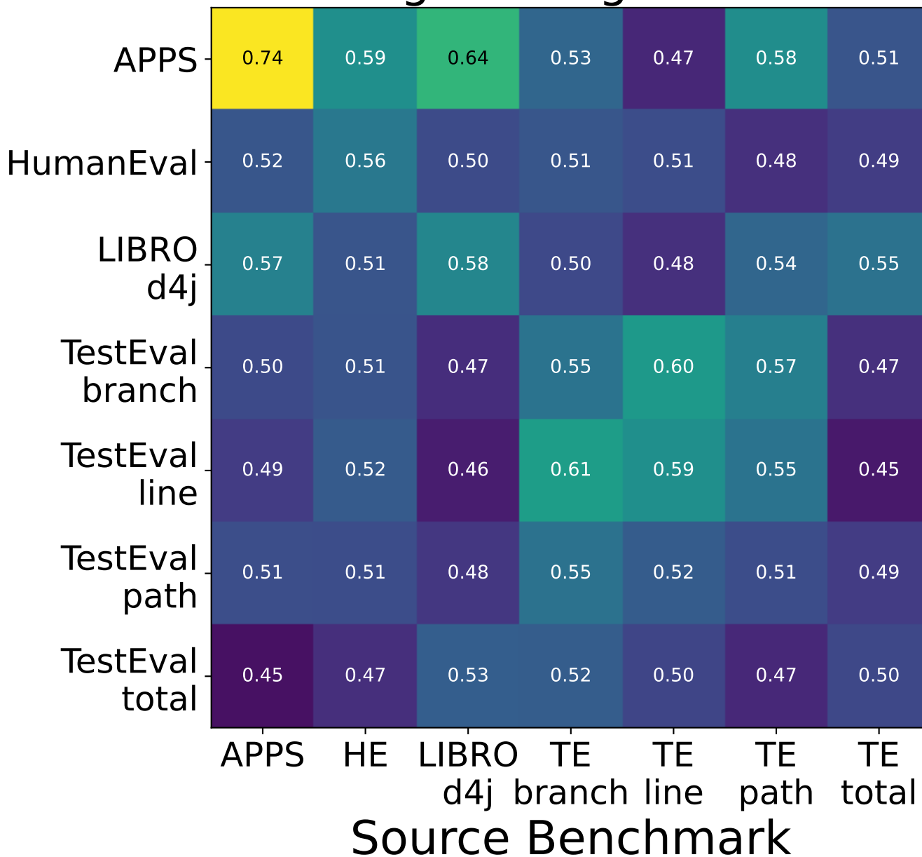
Logistic Regression
