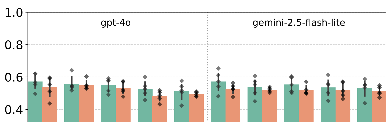
Weak Models
