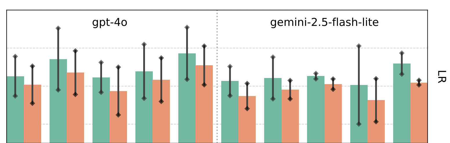
Code Generation
