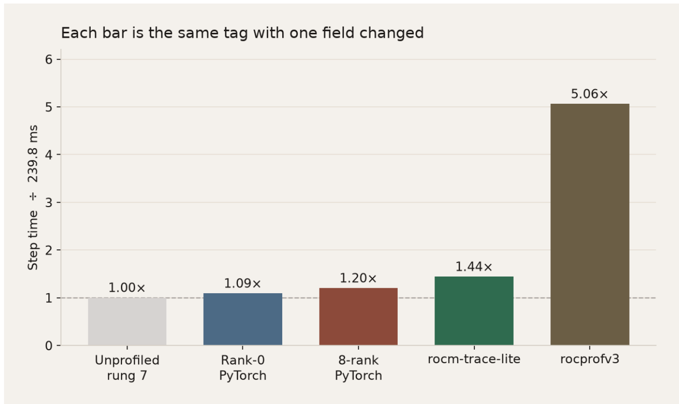
Figure 4. How far each lens moved the step, relative to Table 1. Every bar is the rung-7 madengine run with one field changed. The rank-0 window stays close to the training step, which is why the operator mix below can be read in milliseconds. rocprofv3 is the whole 6-iteration process.
