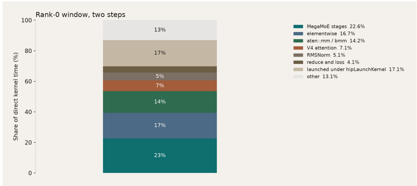
Figure 7. Share of direct kernel time in the rank-0 window. The hipLaunchKernel slice is kernels whose CPU parent is the launch itself. It is already inside the 100 percent, so it is not added on top of the MegaMoE slice.
