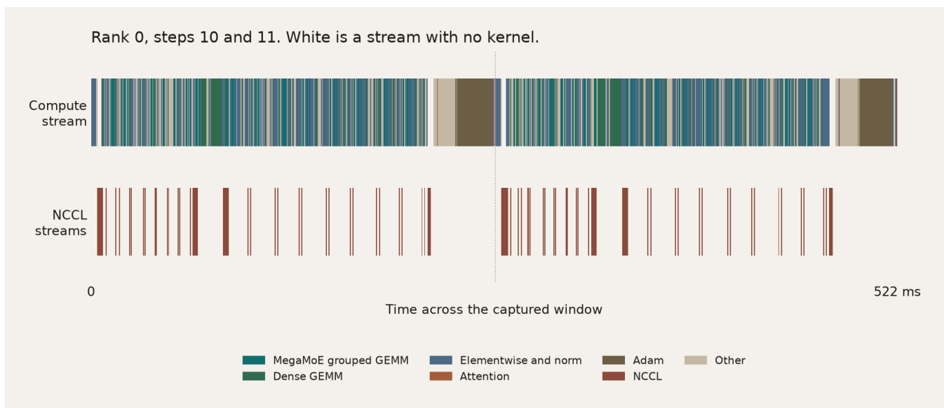
Figure 5. Full captured window, rank 0, steps 10 and 11. White is a stream with no kernel. Each half ends in an Adam block on the compute stream, about 22 ms. NCCL slices sit on the other track and overlap the compute, which is why Table 3's exposed communication is 22.3 ms across both steps while total communication is 58.3 ms. This shape runs one microbatch per rank, so nothing follows that Adam block.
