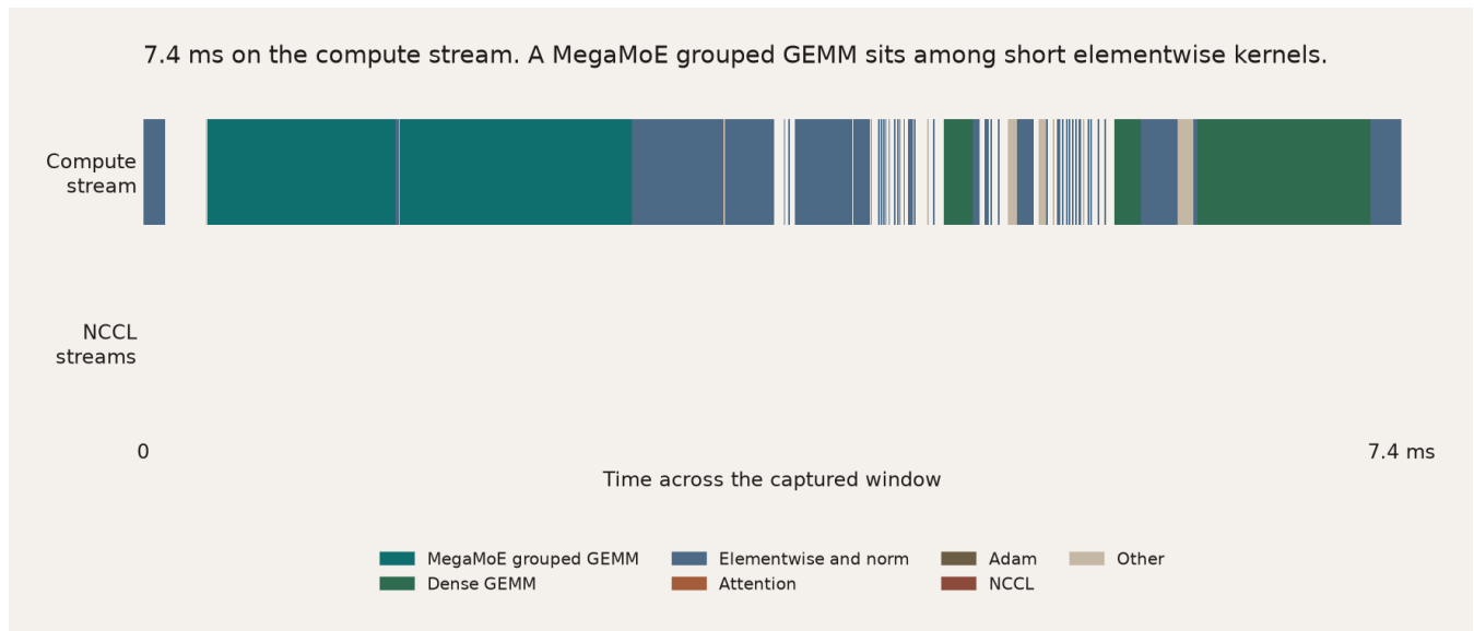
Figure 6. 7.4 ms on the compute stream, 89 kernels. The wide teal slice is dispatch_grouped_gemm_kernel , 1.36 ms. Another teal slice in the same zoom is grouped_gemm_combine_kernel , 1.10 ms. Those are the two kernels the MegaMoE write-up names. The blue slices between them are elementwise, the longest 0.54 ms. A dense GEMM in the same zoom is 0.29 ms. Table 4 is the whole window, not this zoom.
