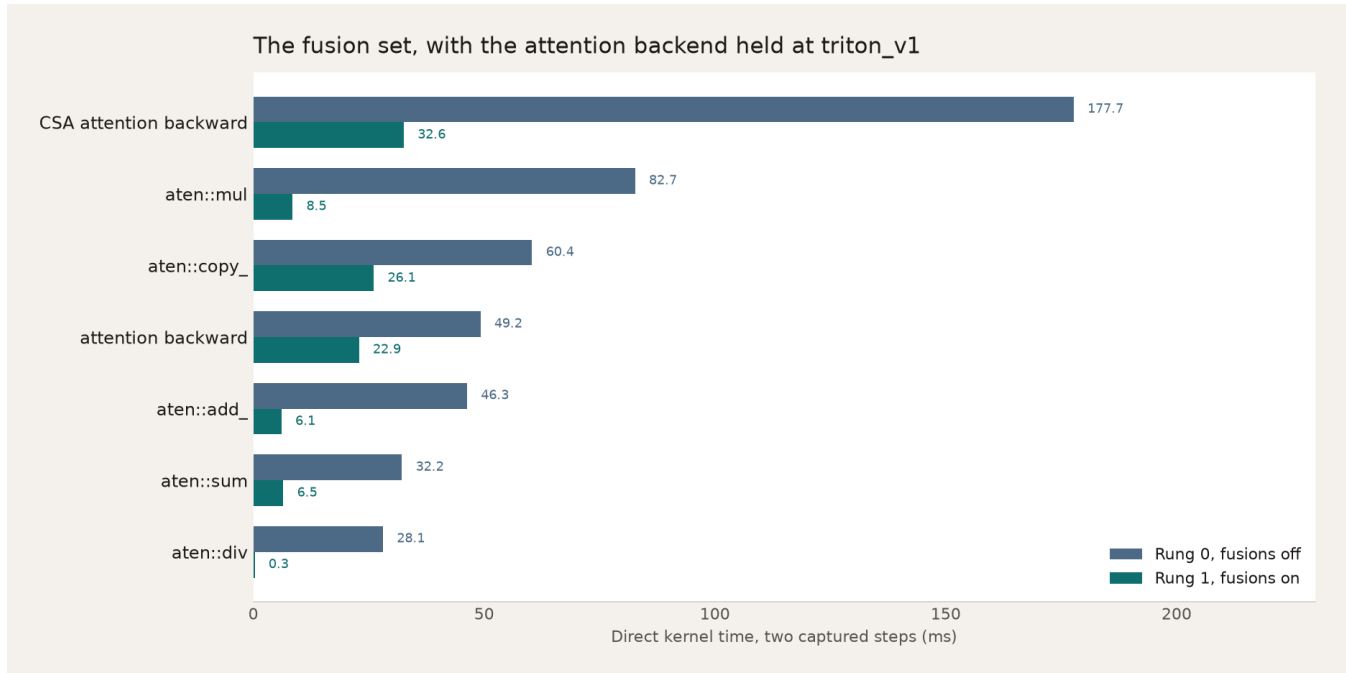
Figure 10. Table 8 as bars. Slate is rung 0. Teal is rung 1. Both totals are two captured steps. The rung-0 window is 1.27× its unprofiled step and the rung-1 window is 1.08×, so a pair of bars does not add up to the 215.5 ms. The attention call counts do not change. _GroupedLinear is off this chart: its forward plus backward stays near 97 ms.
