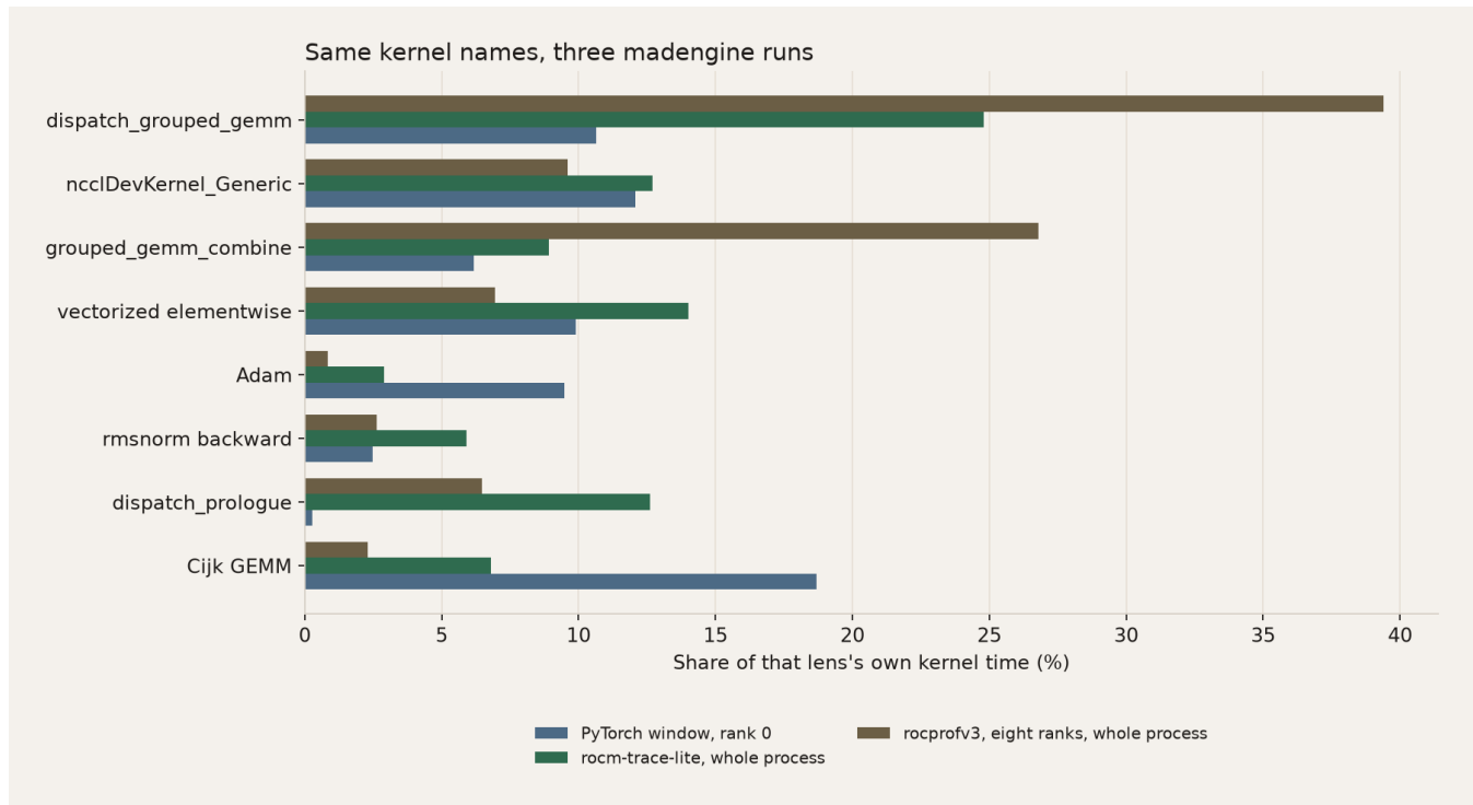
Figure 8. Same kernel names, three runs. The PyTorch bars are shares of kernel time in the 1.09× window. rocm-trace-lite and rocprofv3 are shares of kernel time over the whole process, compile included. dispatch_prologue is 12.6% of the rocm-trace-lite kernel time and 0.3% of the window's kernel time. Cijk GEMMs are 18.7% of the window's kernel time and 2.3% of the rocprofv3 kernel time. The whole-process files confirm the names. The window decides which of those names are in the training step.
