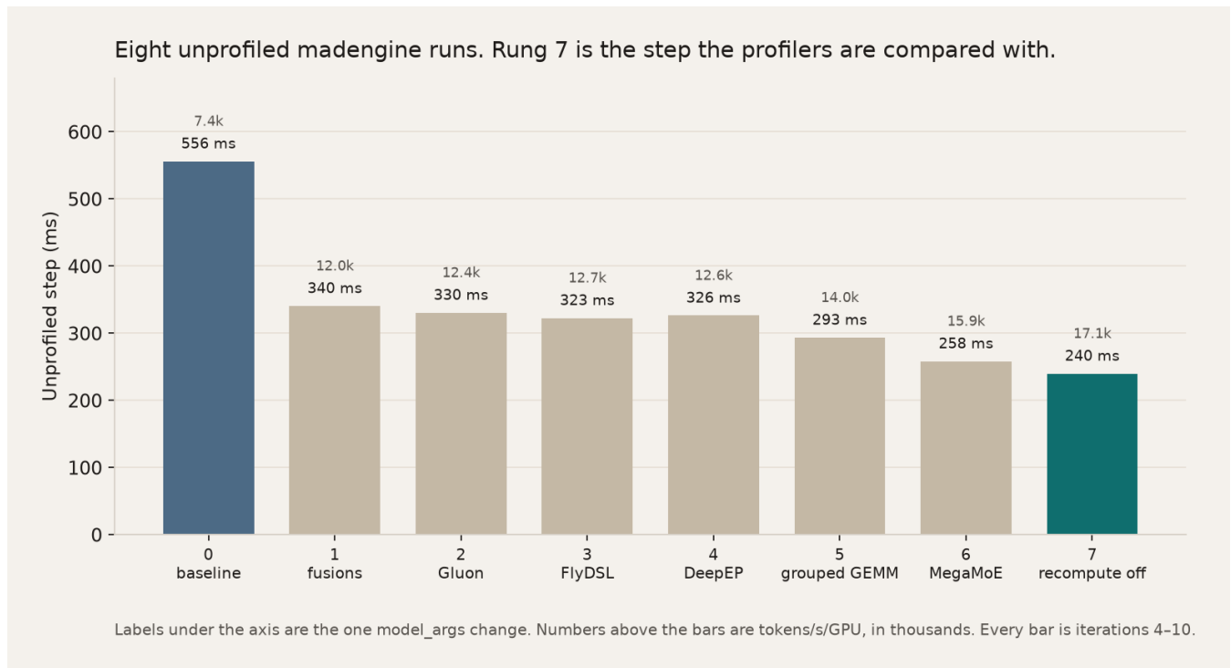
Figure 3. Eight unprofiled runs of one tag. The number above each bar is tokens/s/GPU, in thousands. Rung 7 is the step the later profiler sections use as the training step.
