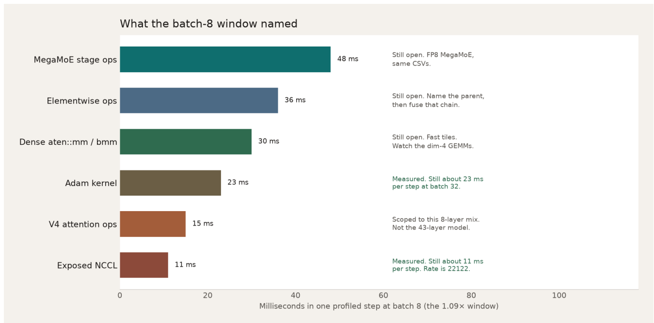
Figure 12. The batch-8 window, one profiled step. MegaMoE, elementwise, and dense GEMM are direct kernel time. Adam is the tail in Figure 5, about 23 ms of that step. Exposed NCCL is about 11 ms of that step, half of the Table 3 bucket because Table 3 covers two steps. The green notes use the same per-step reading of Figure 11. The grey notes are still open.
