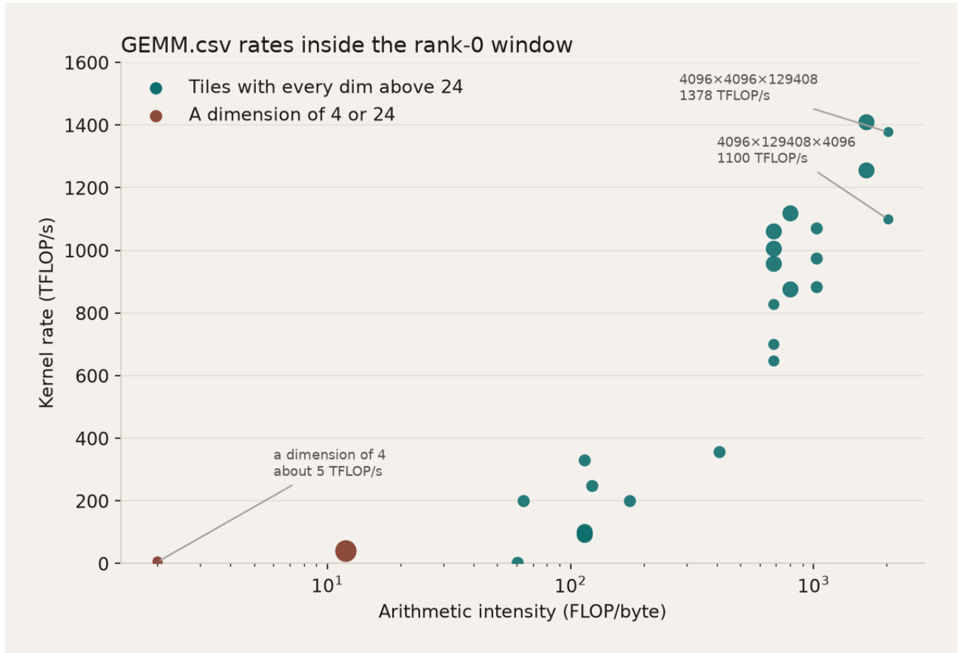
Figure 9. GEMMs TraceLens could model from the rank-0 window. Teal points have every dimension above 24. Brown points have a dimension of 4 or 24. The two tiles at 2016 FLOP/byte run at 1100 and 1378 TFLOP/s. The tiles with a dimension of 4 run at 4.7, 5.1, and 9.3 TFLOP/s. There is no MI350X ridge on this plot: TraceLens has no MI350X peak in this install, and this post does not borrow an MI300X or MI355X peak to draw one.
