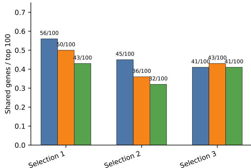
Top-gene overlap
